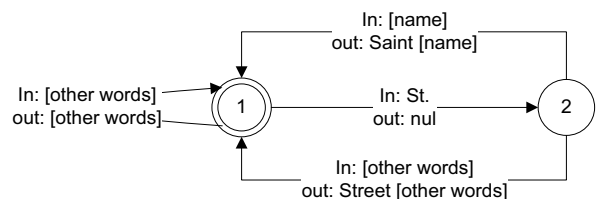
Figure 2: an example FST for text normalization.
