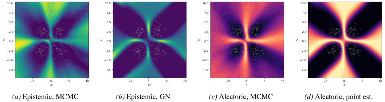
Figure 4. Binary XOR uncertainty maps. Left two panels: epistemic uncertainty (MCMC vs. \|g\|^2 ). Right two panels: aleatoric uncertainty (MCMC vs. point estimate). All maps are individually normalized to [0, 1] .
