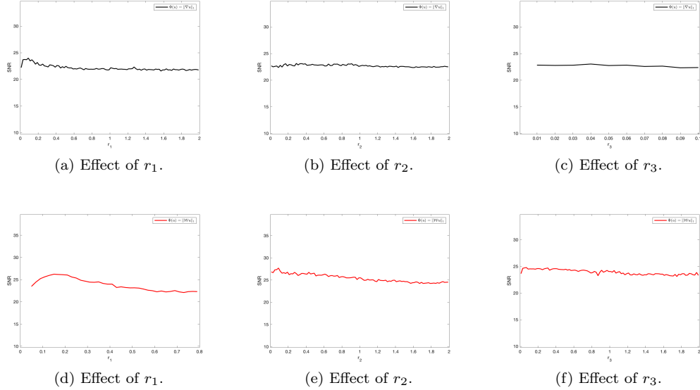
FIGURE 4. Sensitive analysis with parameters r_1 , r_2 , and r_3 . Image ‘cameraman’ with the degradation of the 3n Fourier mask ratio 50% and SNR = 30. The first row displays the results of the proposed model with \Phi(u) = \|\nabla u\|_1 and the second row is the results of the proposed model with \Phi(u) = \|\mathcal{W}u\|_1 .
