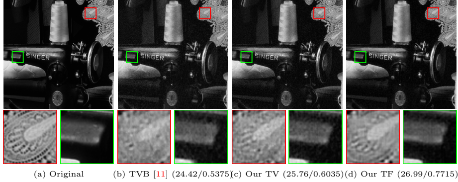
FIGURE 7. The comparison results (SNR/SSIM) of Img08 with 3n Fourier mask ratio 50% and \sigma = 10 .
