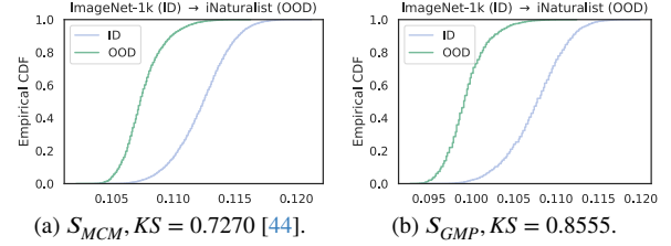
Figure 4. Comparison of (a) S_{MCM} [44] and (b) our S_{GMP} on ImageNet-1k (ID) to iNaturalist (OOD). The scores are multiplied by 100 for better illustration. KS is the Kolmogorov–Smirnov statistic. Higher KS values indicate a greater difference between the distributions. Best viewed in color.
