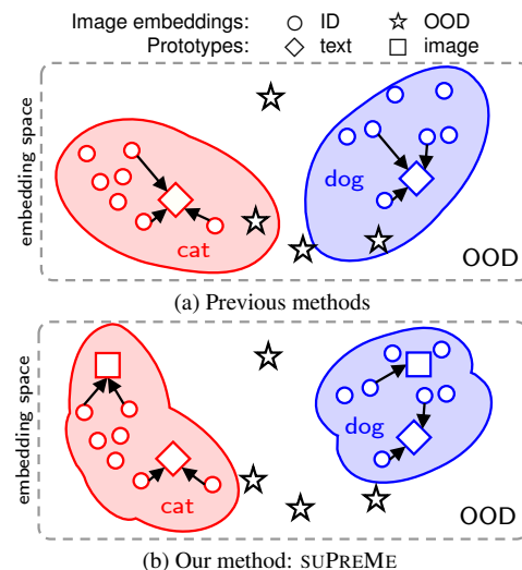
Figure 1. (a) Previous VLM-based OOD detection [36, 44, 45] uses only ID text prototypes ( \diamond ) to identify OOD samples. (b) SUPREME employs ID image prototypes ( \square ) to complement ID text prototypes, reducing the impact of the image-text modality gap [39] and sharpening the boundary between ID and OOD.
