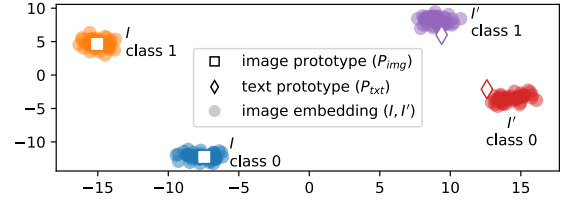
Figure 5. The t-SNE visualization of embeddings from two arbitrary classes in ImageNet-1k (Val) using SUPREME.
