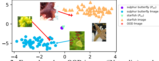
Figure 2. Examples where OOD images (iNaturalist) are located closer to ID text prototypes compared to ID images (ImageNet-1k) generated by CLIP (ViT-B/16). We also visualize the embeddings generated by our SUPREME in Fig. 5, which has smaller gaps between image and text embeddings.
