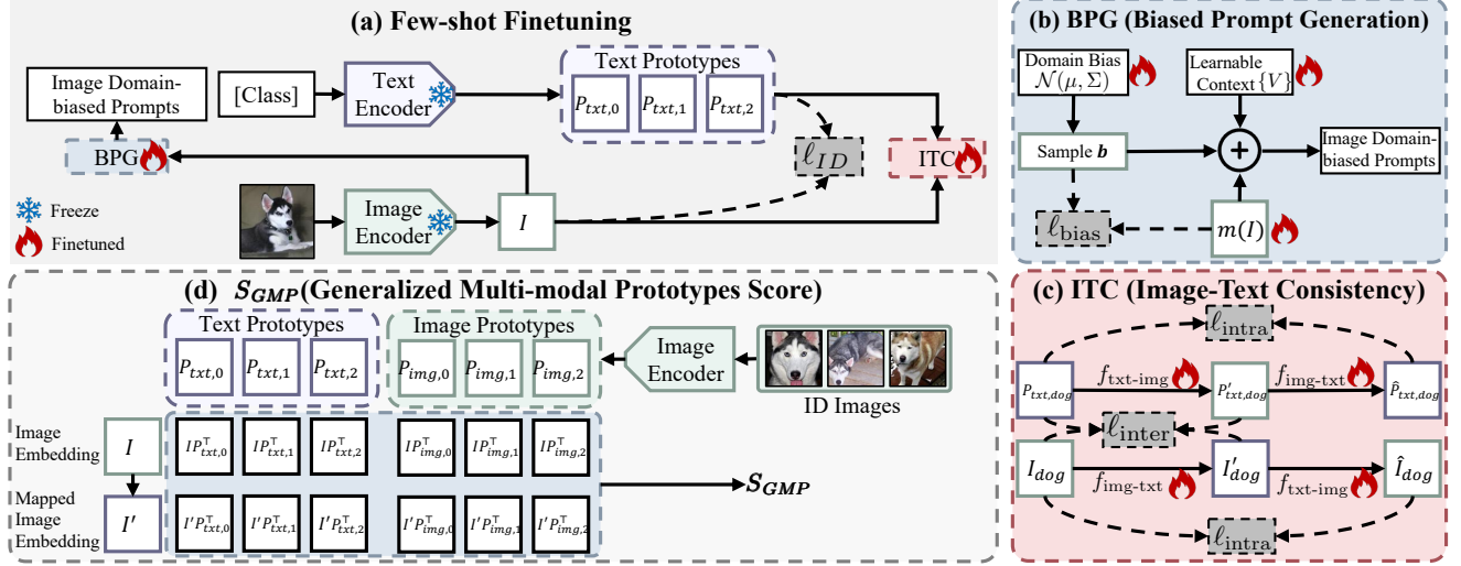
Figure 3. Overview of SUPREME. The two novel modules, i.e. , BPG (biased prompt generation) and ITC (image-text consistency), are designed to minimize the modality gap. (a) During the few-shot fine-tuning stage, (b) BPG generates image domain-biased prompts, conditioned on the estimated image domain bias and the mapped image embedding m(I) for better image-text fusion. (c) ITC minimizes the modality gap directly by the intra- and inter-modal losses ( \ell_{intra} and \ell_{inter} ) with the text-to-image mapping f_{txt \rightarrow img} and the image-to-text mapping f_{img \rightarrow txt} . (d) During inference, image prototypes are obtained by averaging each class’s base ID image embeddings (Eq. (3)). The proposed S_{GMP} (Eq. (10)) is calculated based on the maximum similarity between the multi-modal embeddings (the image embedding I and mapped image embedding I' ) and ID multi-modal prototypes ( i.e. , text prototypes \{P_{txt,c}\}_{c=1}^C and image prototypes \{P_{img,c}\}_{c=1}^C ). S_{MCM} refers to the MCM score [44].
