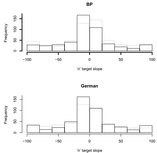
Figure 3: Histograms for target slope (st/s) for BP (top) and German (bottom) for the non-prominent label. Plain line is ST style and dotted line, RE style.
