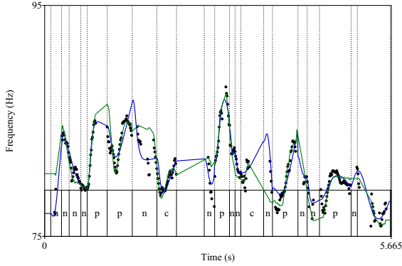
Figure 2: F_0 traces in st re 1 Hz for the Fujisaki (green) and the qTA models (blue) for the read sentence: “Was ihn aber am meisten Überwindung kostete war (c), sich mitten in der Nacht(c) zu erheben , um das Morgengebet zu sprechen (t).” by German male speaker G1. See text and Fig. 1 for further details. Audio files: G01-3Orig.wav, G01-3Fuji.wav, G01-3qTA.wav
