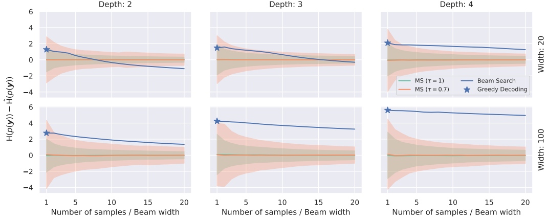
Figure 4: Estimator of Predictive Entropy. Results for different vocabulary sizes (width) and sequence lengths (depth). We estimate the entropy H(p(\mathbf{y})) using N Monte-Carlo samples (cf. Eq. (5)). Lines denote the average over runs, while shades denote one standard deviation. We compare MS for two commonly used \tau . The experiments show that the decreased temperature leads to lower variance but introduces bias.
