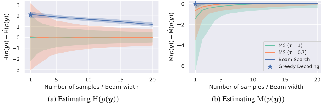
Figure 1: Quality of estimators for synthetic predictive distributions p(\mathbf{y}) with |\mathcal{V}| = 20 and T = 4 . The predictive entropy H(p(\mathbf{y})) is estimated as in Eq. (5) using multinomial sampling (MS) with different temperatures ( \tau ). The negative maximum sequence log-likelihood M(p(\mathbf{y})) is estimated by the maximum over N samples obtained by beam search ( N = 1 represents greedy decoding) or MS with different \tau . Statistics are obtained by sampling 2000 different p(\mathbf{y}) . (a) Lines show average, shades denote one std. (b) Lines show the median, and shades denote the 5% to 95% quantile range.
