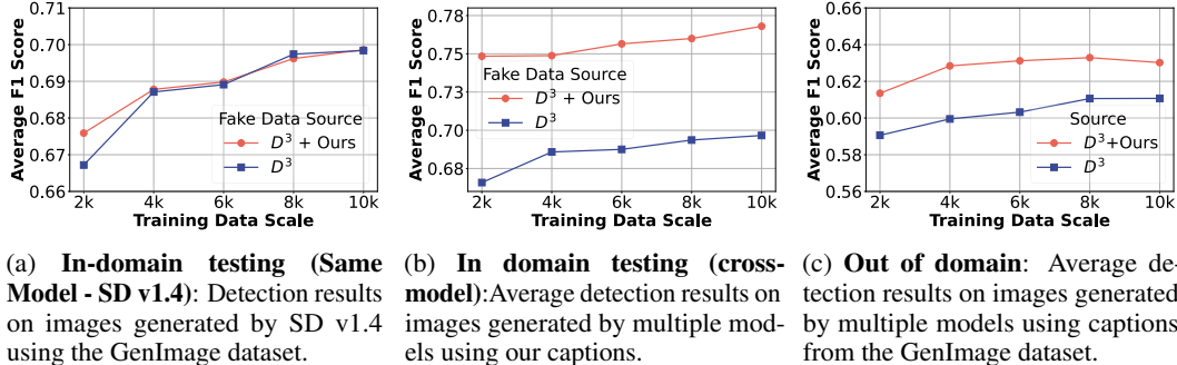
Figure 6: Results for Application 4: Generated content detector. Comparison of detection performance across different data scales using D^3 alone versus the combined D^3 + GENERATE ANY SCENE training set in cross-model and cross-dataset scenarios.
