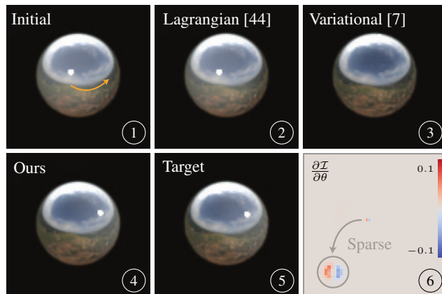
Figure 1. Image gradients are sparse with respect to optimization parameters that induce motion in the image space ⑥. We show an inverse problem with the goal of recovering the position ( \theta ) of a distant light source from a synthetic image of a shiny ball, i.e. ① to ⑤. Existing methods compute proxy gradients such as: Lagrangian derivatives [44], which track only primary-ray intersections, or variational derivatives [7], which can be prone to local minima. Our method uses standard RGB gradients and uses an inverse rendering objective that matches locally orderless images.
