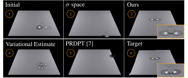
Figure 9. Using a real photograph. We show a preliminary experiment with real data that validates our method’s robustness against sensor noise and calibration errors. Starting with known material, camera, and lighting, and a randomly positioned glass orb ①, we recover the optimal translation from a real photograph ⑥ using variational optimization. The variational estimate with 8 samples is shown in ④. Matching at stationary resolution ⑤ or only in the \sigma space ② fails in this task. Our method achieves optimal recovery starting from any initial position on the surface.
