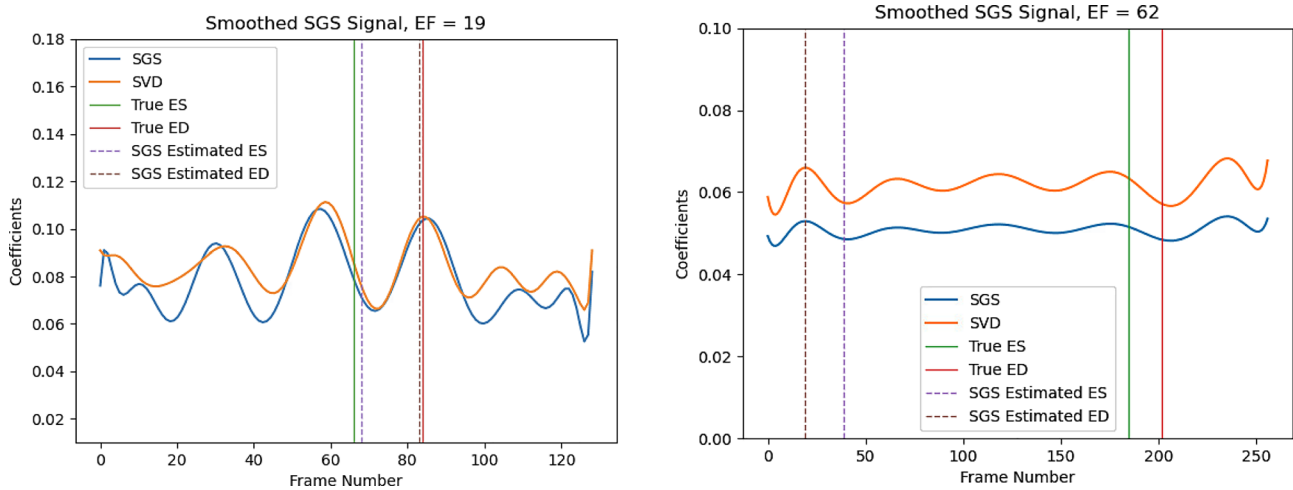
Fig. 4 Example for ED/ES detection by SGS EchoNet. Peaks are identified using original, un-smoothed coefficients
