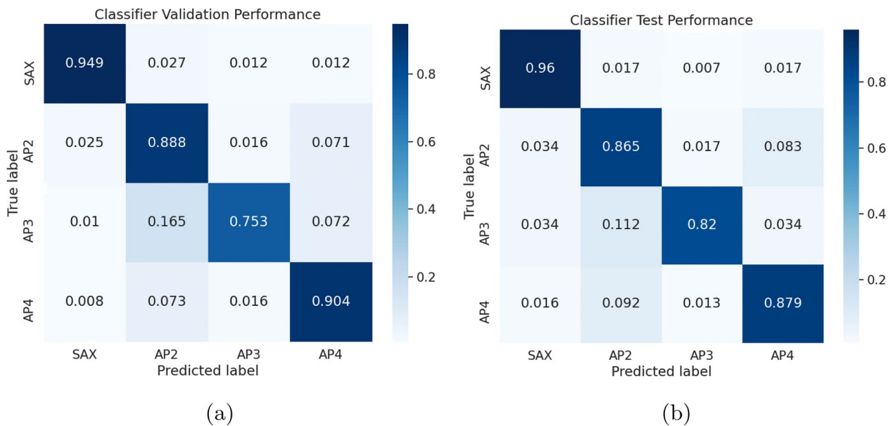
Fig. 3 Confusion matrices for PROMISE echo view classification normalized by row indicating true view classification rates. Validation accuracy (left): 0.90. Test accuracy (right): 0.89
