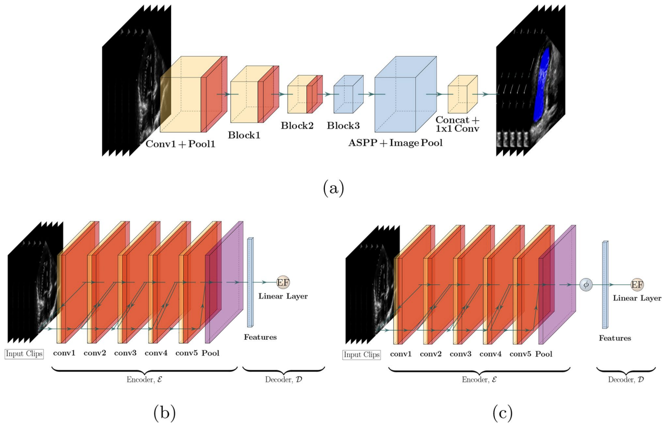
Fig. 2 Model diagrams. EchoNet dynamic consists of two arms: (a) a DeepLabV3 encoder for LV segmentation and (b) an R(2+1)D encoder followed by spatiotemporal pooling for EF estimation. The segmentation model is used to identify and feed clips of the cardiac cycle to the EF estimation model. When we use EchoNet dynamic without its segmentation model for clip selection, it is identical to (b) and we refer to it as EchoNet No-seg. (c) Spectral EchoNet also uses a R(2+1)D encoder, but followed by spatial pooling and frame-level aggregation, \phi . Note that we allow \phi to be a composition of frame-level aggregation and a transformation of the aggregated features. In Sect. “Spectral and scaled Gumbel-Softmax EchoNet”, we choose an SVD decomposition for frame-level feature aggregation and then a smooth transformation of those features (see Eq. (3) and its discussion). Finally, all EF models use a linear layer after pooling
