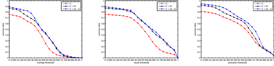
Figure 13: Comparison of the performance of trackers which make use of one, two and three-level clustered decision trees, where the successive tree levels exploit colour, motion and depth features respectively. Graphs show the success ratio versus overlap threshold curve for each tracker, when tested on five RGB-D sequences from a public benchmark data set. C, M, D denote colour, motion and depth features respectively.
