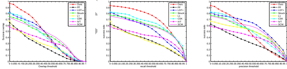
Figure 8: The success ratio versus overlap threshold, recall threshold and precision curves in 18 sequences with illumination change.
