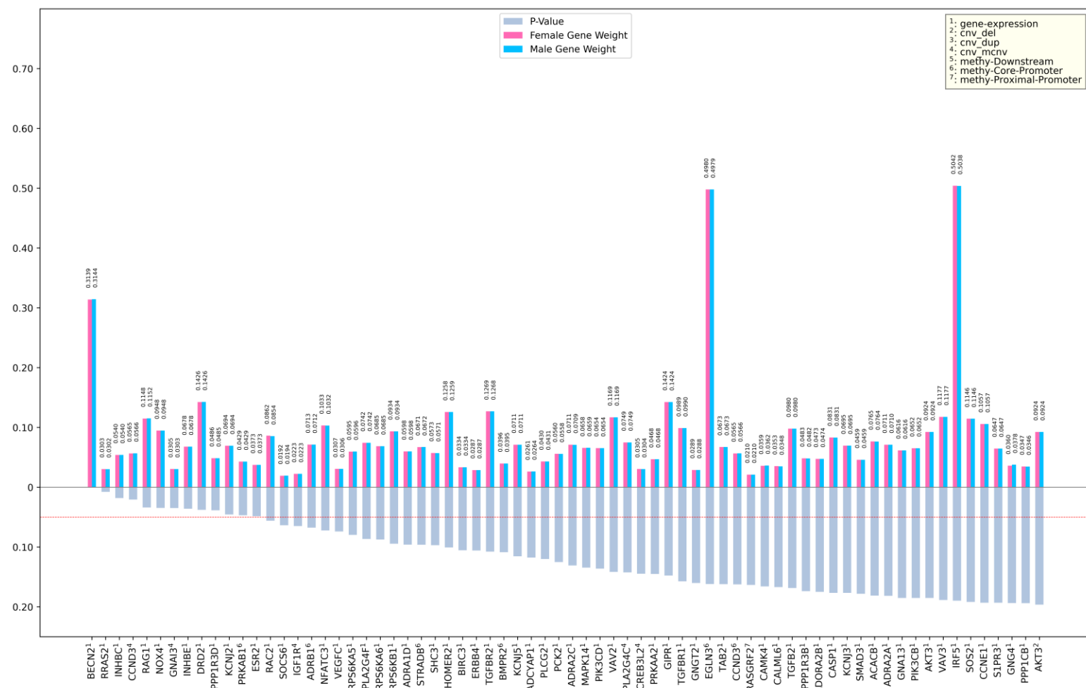
Figure 7. Bar chart displaying the weight of important genes in female and male, ranking by their p-values. (The red dashed line indicates a p-value threshold of 0.05)
