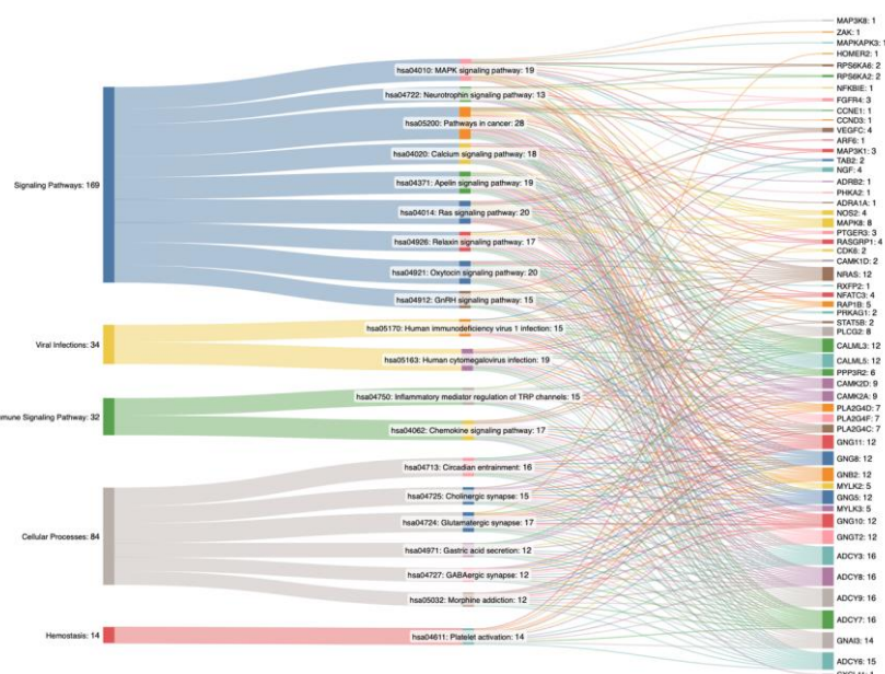
Figure 9. Sankey diagram illustrating the relationship between the identified signaling pathways and corresponding genes using the top 70 genes features found to be associated with AD
