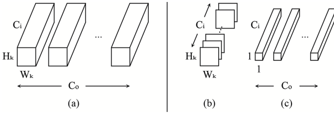
Fig. 2. (a) Standard convolutional filters are factorized into (b) depth-wise convolutional filters for intra-channel convolution and (c) point-wise convolutional filters for cross-channel projection.
