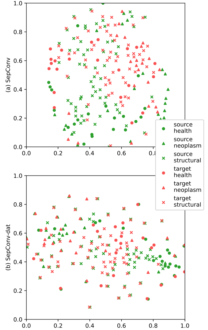
Fig. 6. The t-SNE plots of the latent features extracted by the feature extractor in (a) the SepConv and (b) the SepConv-dat . The data in the source domain are marked in green, whereas the data in the target domain are marked in red.
