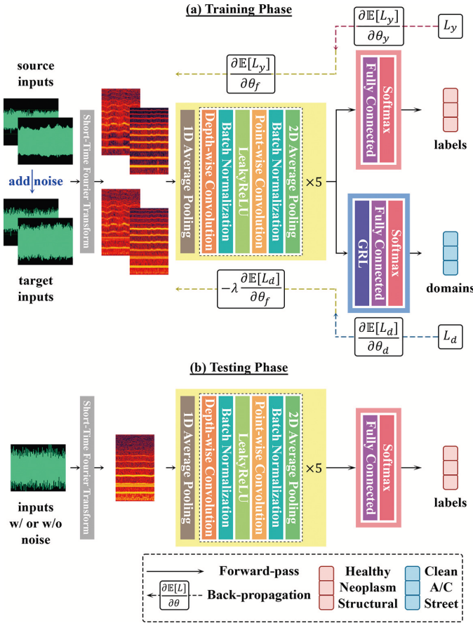
Fig. 1. The feature extractor consists of 5 separable convolutional blocks; The disease predictor and domain classifier are simply combinations of a fully connected layer and a softmax layer.
