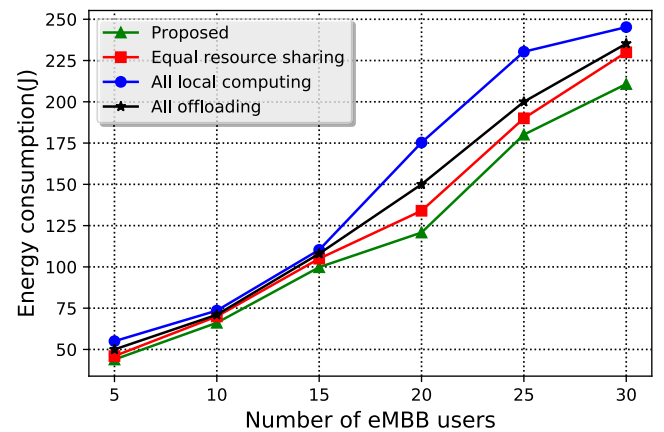
FIGURE 6. Energy consumption under different number of users.
