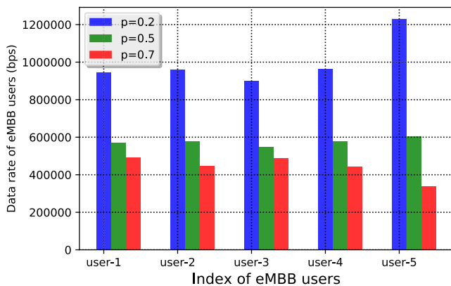
FIGURE 12. Achieved data rate of eMBB users.
