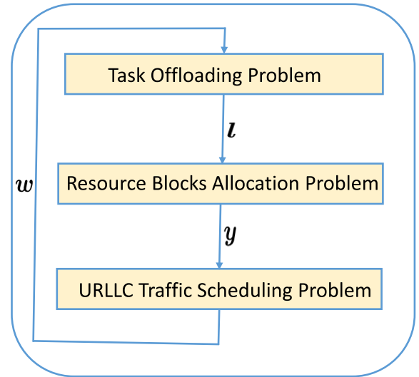
FIGURE 3. Optimization framework.
