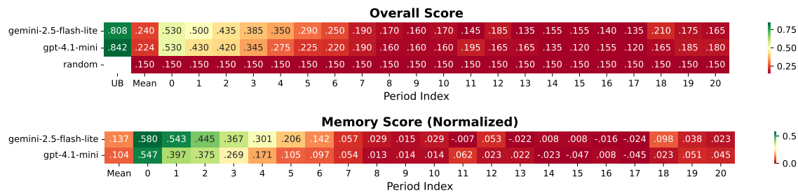
Figure 12: Memory evaluation results on the extra configuration.
