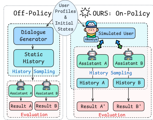
Figure 1: On-policy v.s. off-policy evaluation for assistants’ memory.
