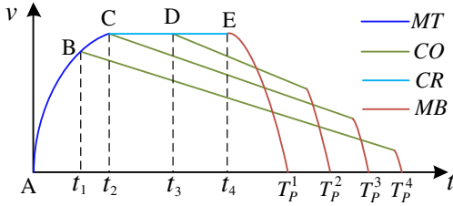
Fig. 5. Schematic diagram of the optimal strategy trajectories
