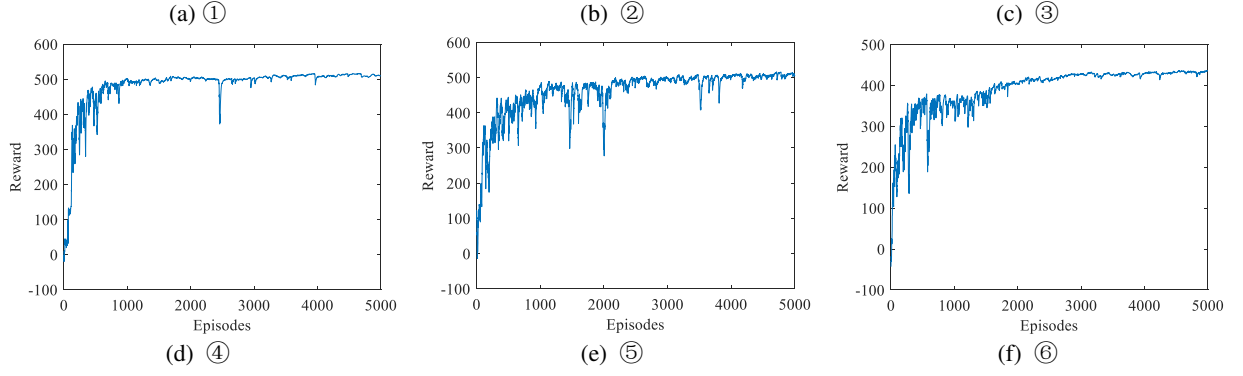
Fig.8. The convergence curves S-PPO and PPO based on relaxed dynamic reward, average dense reward and sparse reward
