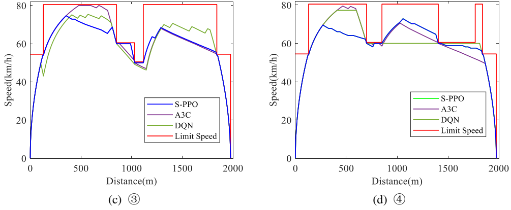
Fig. 12. The trajectories of train operating under various speed limit using S-PPO, A3C, and DQN
