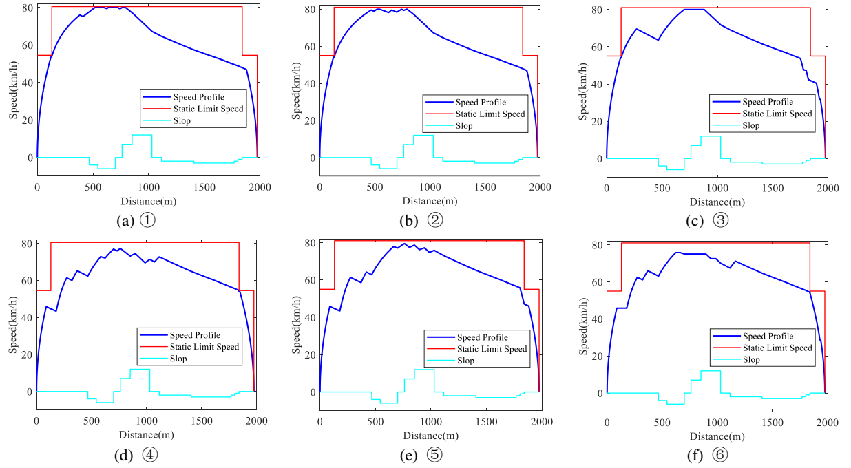
Fig.9. The trajectories of train operating using S-PPO and PPO based on relaxed dynamic reward, average dense reward and sparse reward
