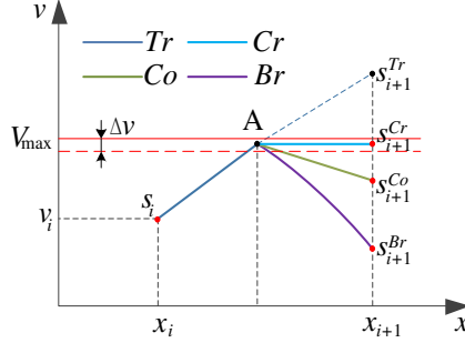
Fig.2. Rechoosing plan for a constant speed limit interval
