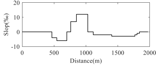
Fig.7. The slope data of the track
