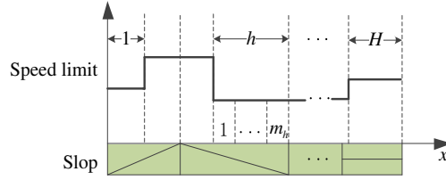
Fig. 1. The principle of track discretization
