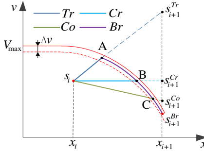
Fig.3. Rechoosing plan for the braking speed limit interval
