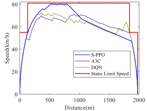
Fig.11. The trajectories of train operating comparison among the three algorithm
