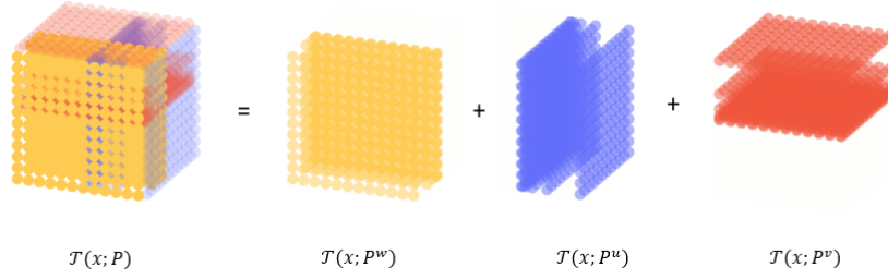
Figure 9: Illustration on arranging a full sparse volume into three compact volumes. Let the phasor volume with zero frequency centered. We selectively mask out some entries of the phasor volume as zero, then approximate the spatial feature embedding of a large phasor volume in terms of the sum of the embedding from three smaller ones, each of which dilates along an axis. Despite there are some overlap entries, e.g. , the center entry appears in all three tiny volumes, it will not affect the performance as it is an over-parameterization. The three compact volumes can be reparameterized back to the original single full volume for conducting Fourier multiplication, such as level-of-detail filtering. The complete transformation from phasor volume to spatial feature embeddings is shown in the PyTorch pseudo-code in Algorithm 1.
