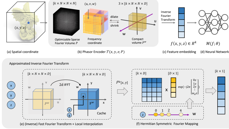
Figure 2: Pipeline of PREF. We model the underlying sparse frequency representation of the scene (b) and augment it with neural network (d) to achieve full spectrum recovery. The inverse Fourier transform is approximated by two consecutive sub-procedures (e) and (f).
