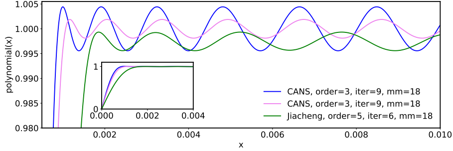
Figure 4. Comparison of CANS polynomials with (Jiacheng, 2024).
