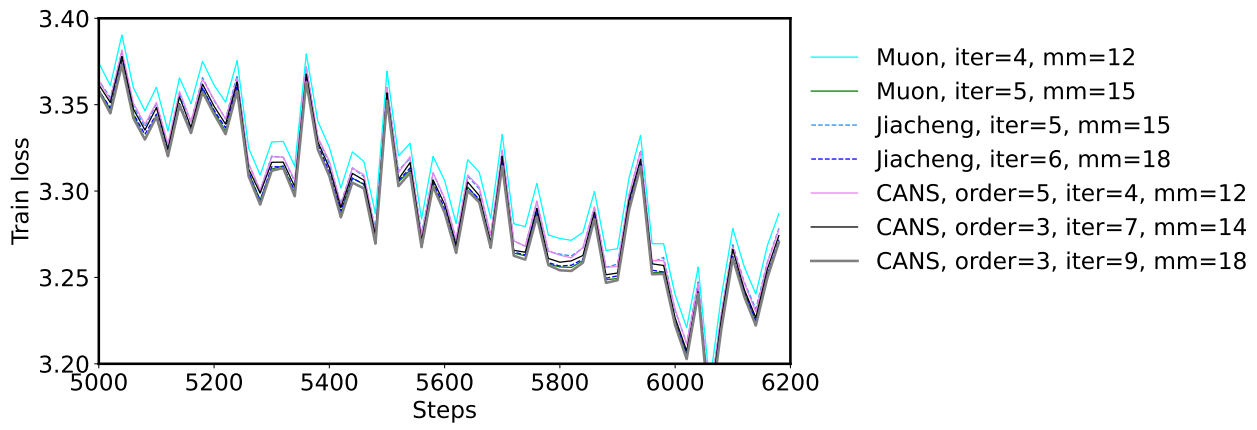
Figure 9. NanoGPT smoothed train loss curve.
