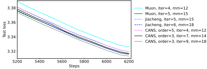
Figure 5. Test loss of NanoGPT trained using Muon optimizer with different polynomials.
