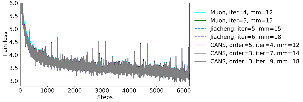
Figure 7. NanoGPT full train loss curve.
