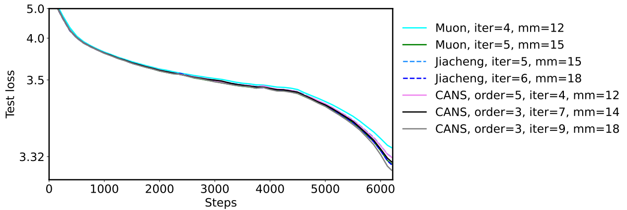
Figure 8. NanoGPT full test loss curve.
