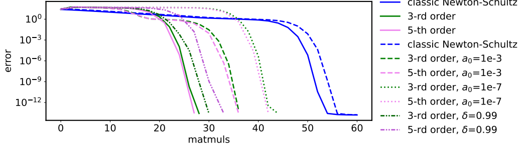
Figure 2. Convergence of iterative algorithms for matrix orthogonalization. The solid lines show the performance when the exact values of \sigma_1(A) , \sigma_n(A) are known, and the matrix is normalized by \sigma_1(A) . In other cases, the matrix is normalized by \|(A^T A)^2\|_F^{1/4} and the precise value of the left boundary is \sigma_n(A)/\|(A^T A)^2\|_F^{1/4} = 9e-5 . The striped lines show performance for overestimated boundary a_0 = 1e-3 , the dotted lines – for underestimated a_0 = 1e-7 . The dashdotted lines show convergence of algorithm with 4 iterations of \delta -orthogonalization (Algorithm 2).
