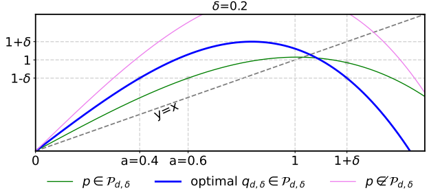
Figure 1. Illustration of the selection of a degree-3 ( d = 2 ) polynomial with a large derivative at zero. The green polynomial falls into [1 - \delta, 1 + \delta] , but has insufficient derivative. The blue polynomial q_{d,\delta} has the highest possible derivative among polynomials from \mathcal{P}_{d,\delta} . The purple polynomial is not part of \mathcal{P}_{d,\delta} , and its derivative is too large.
