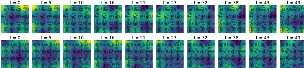
Figure 4: Imputed results on 2D Shallow Water dataset where 30% of the original data points are available for training.
