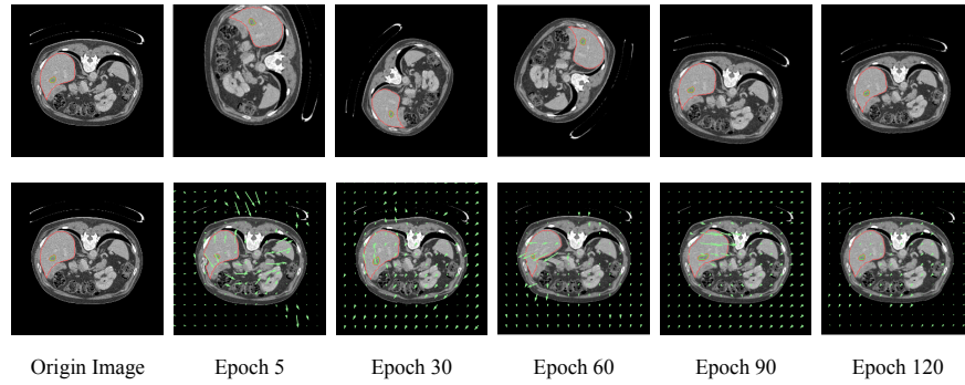
Fig. 3: Visualization of two augmentation modules: A-STN ( top ) and D-VAE ( bottom ). Red line is the contour of liver while green line is the contour of tumor. Our OnlineAugment can generate diverse augmented images. Moreover, it can also adapt to the target network. As the target network converges during training, the magnitude of the augmentation will also decrease.
