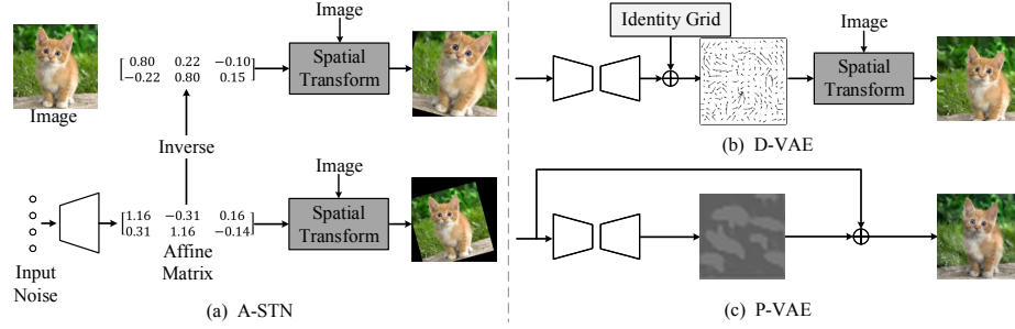
Fig. 2: Augmentation models: A-STN (a), D-VAE (b), and P-VAE (c). A-STN, conditioned on Gaussian noise, generate a transformation matrix. Both the matrix and its inverse are applied to an image for diversity. D-VAE or P-VAE takes an image as input, generating deformation grid maps or additive noise maps. The three models are trainable if plugged in the training scheme in Figure 1.
