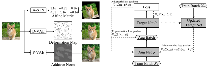
Fig. 1: Augmentation illustrations ( Left ) and OnlineAugment scheme ( Right ). We propose three models to conduct spatial transformation, deformation, and noise perturbation. OnlineAugment can jointly optimize each plug-in augmentation network with the target network. Updating the augmentation network incorporates adversarial training, meta-learning, and some novel regularizations.
