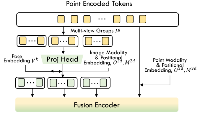
(b) Model architecture of 3D to multi-view encoder.
