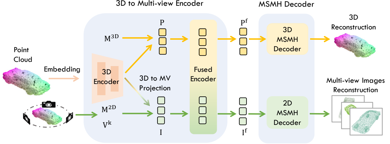
Figure 1. Overview of the stage one training process of the teacher model. The input point clouds are first encoded into intermediate 3D tokens using a 3D encoder. Leveraging the provided pose information, these tokens are projected onto multi-view (MV) 2D image tokens through our proposed view-based feature projection method. Modality and pose embeddings are then added to both the projected 2D tokens and the intermediate 3D tokens. These tokens are concatenated and refined by a multi-modal fusion module. Finally, the refined features are fed into two separate decoders that independently reconstruct the complete multi-view 2D images and the 3D point clouds.
