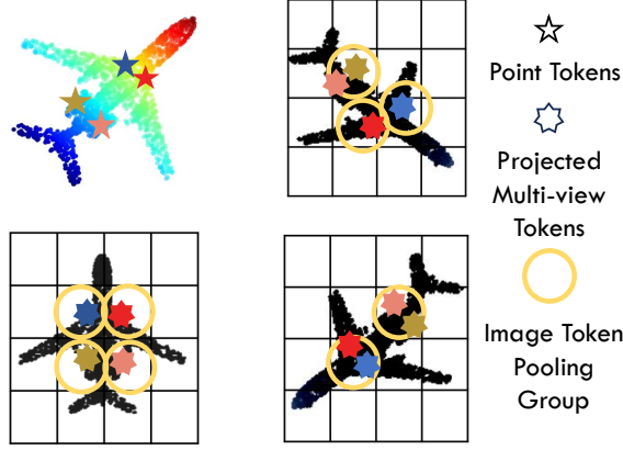
(a) 3D to multi-view tokens-level projection.
