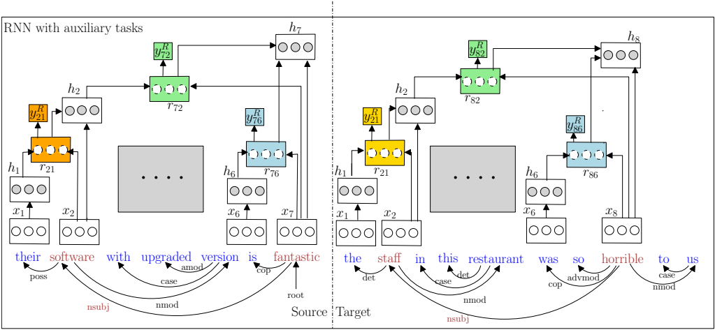
Figure 5 An example of RNN with auxiliary tasks for both source and target domains.
