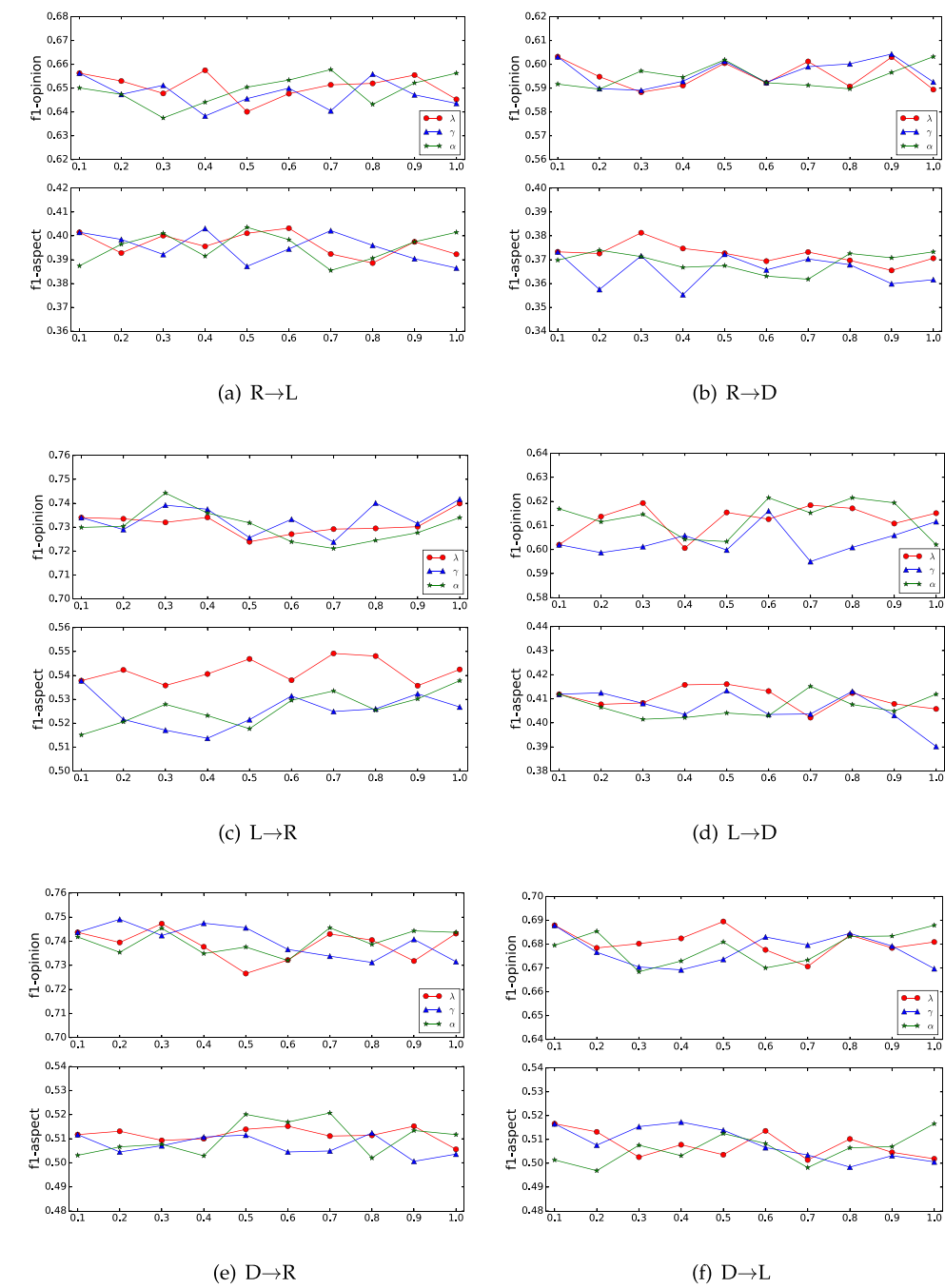
Figure 9 Sensitivity studies for \lambda , \gamma , and \alpha on six different transfer experiments.
