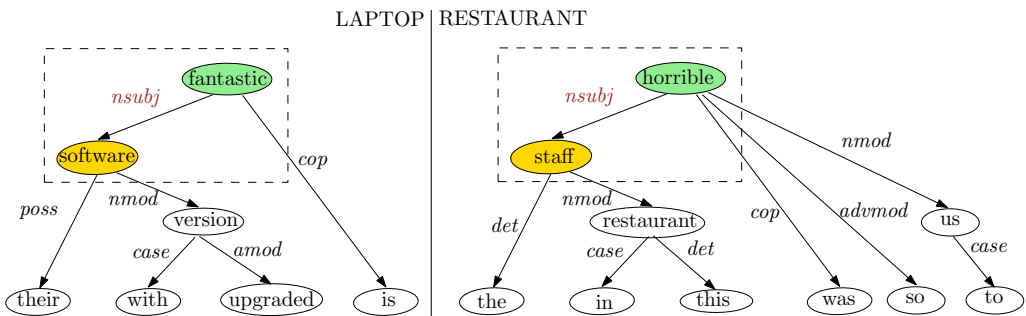
Figure 1 An example of two reviews in different domains with similar syntactic patterns.
