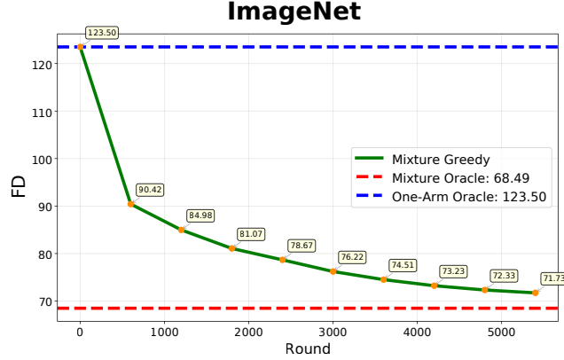
Figure 4. Convergence of FD in ImageNet dataset generative models.
