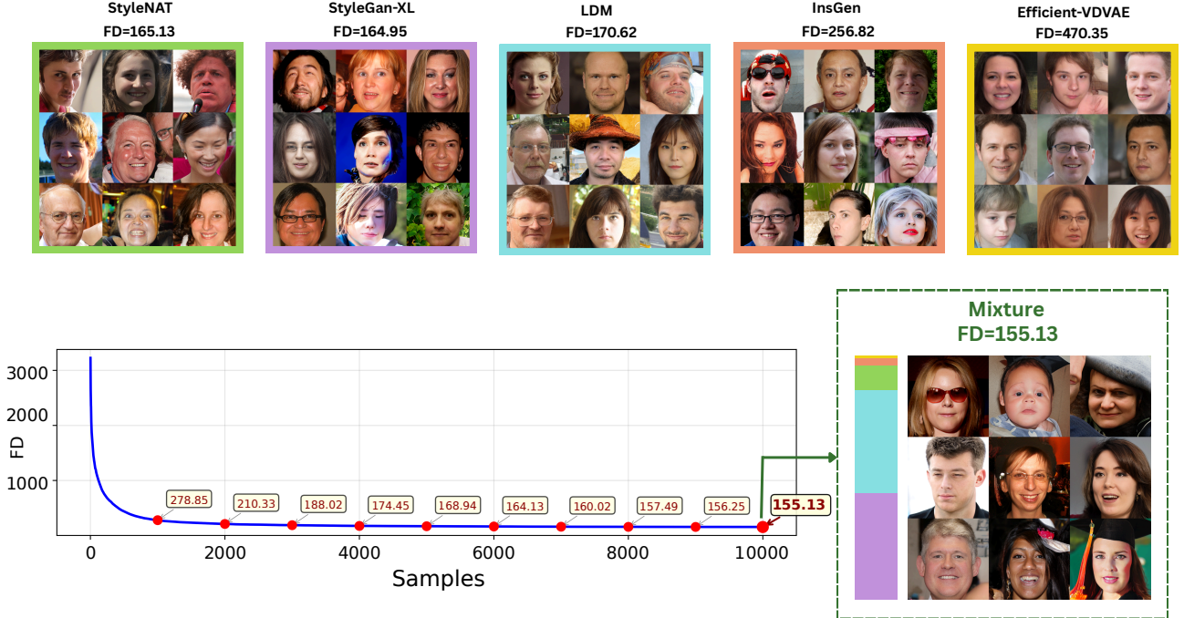
Figure 3. Mixture Greedy, minimizing Frechet Distance using exponentiated gradient descent on FFHQ generated samples.
