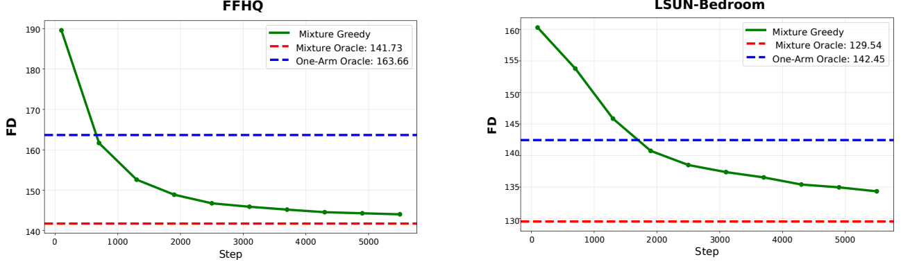
Figure 2. Convergence of Mixture Greedy in terms of Fréchet Distance (FD) across image selection steps on FFHQ and LSUN-Bedroom.
