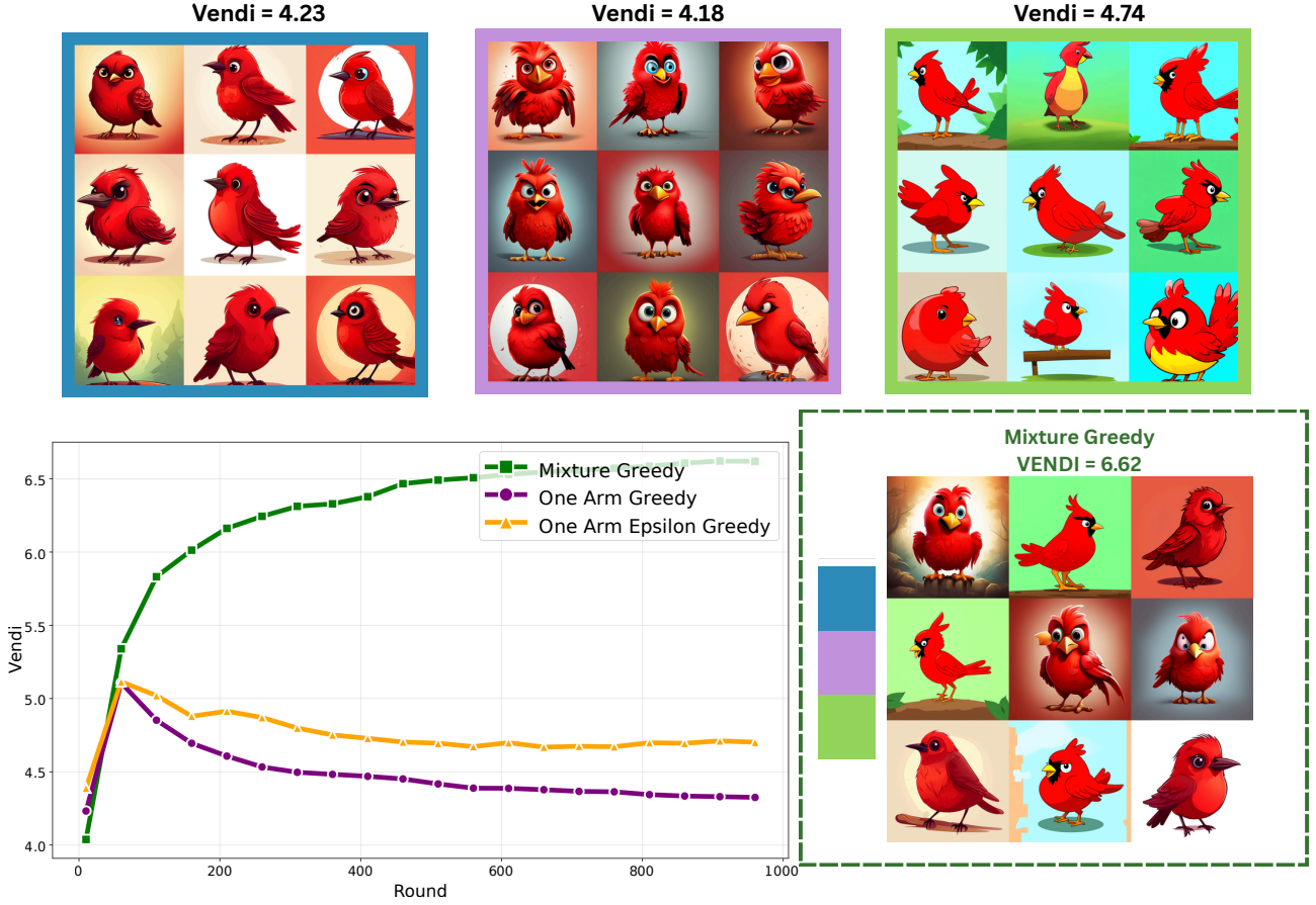
Figure 5. Application of Mixture Greedy on the generated red birds dataset to optimize Vendi Score.
