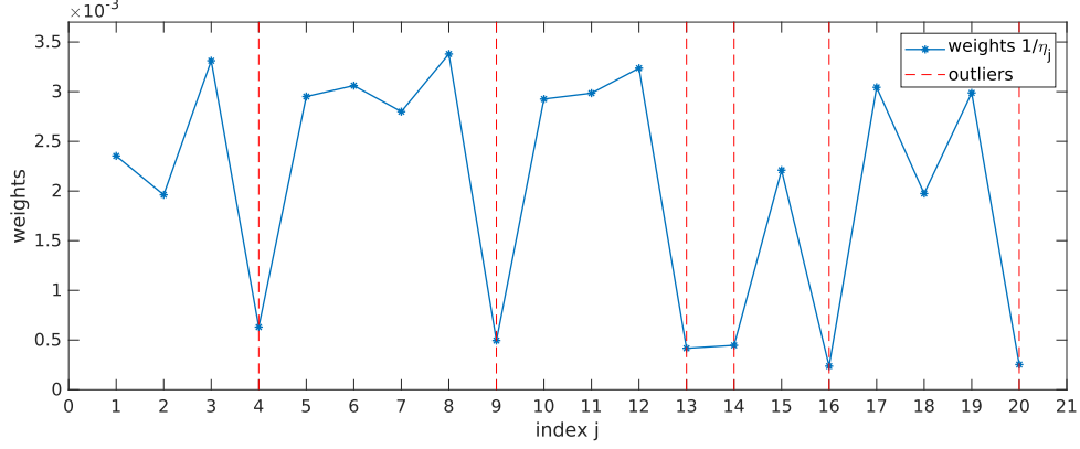
Figure 13: Weights of the IRLS procedure. We synthesized a sequence u_0 containing L = 20 low-resolution images using a sequence of displacements \delta . Then, we computed a perturbed sequence of displacements \delta' using two levels of perturbations: 70% of the displacements were perturbed using a Gaussian noise with a small standard deviation \sigma_1 = 0.01 while 30% of them were perturbed using a Gaussian noise with a large standard deviation \sigma_2 = 0.3 . We display using blue-marks the weights w_j = 1/\eta_j ( 1 \leq j \leq L ) obtained using the IRLS procedure (56) over the sequences u_0 and \delta' . We indicate using red-dashed lines the indexes of the outliers in u_0 , that is, the indexes j of the elements of \delta' undergoing a large perturbation. As we can see, those outliers are associated to significantly low values of w_j compared to the others.
