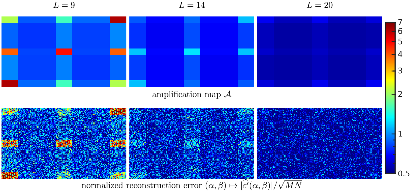
Figure 4: Amplification map and reconstruction error in the Fourier domain. First row: the amplification map \mathcal{A} defined in Proposition 6, for different values of L , \sigma = 1 , random i.i.d. \mathcal{U}([-5, 5]^2) translations and super-resolution factors equal to z_x = M/m = 129/56 \approx 2.3 and z_y = N/n = 73/33 \approx 2.2 respectively. Second row: the corresponding normalized reconstruction error |\widehat{\varepsilon}'|/\sqrt{MN} in the Fourier domain (for one realization of \varepsilon ). We can see that the amplification map gives a good prediction of the fluctuations of |\widehat{\varepsilon}'| , and that the amplitude of these fluctuations quickly decreases when L increases. When L is close to z_x z_y (left column), the amplification map may present strong variations from one region to another, which leads to the appearance of some textured error patterns in the reconstructed image (see Figure 5). In most practical cases however, one has L \gg z_x z_y and the amplification map \mathcal{A} is almost constant (and takes small values).
