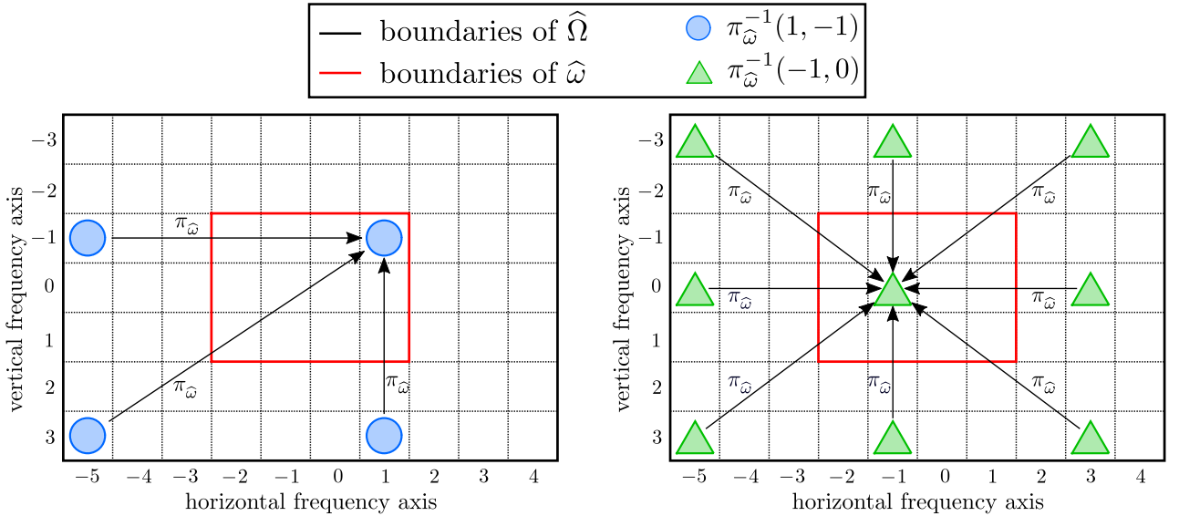
Figure 3: Frequency aliasing with fractional aliasing factors. When a high resolution image with size M \times N = 10 \times 7 is subsampled into a low resolution image with size m \times n = 4 \times 3 using the S_z operator (with z = (z_x, z_y) = (\frac{10}{4}, \frac{7}{3}) ), frequency aliasing occurs. We illustrate here with two examples how the alias function \pi_{\hat{\omega}} involved in Proposition 1 maps the corresponding high-frequency domain \hat{\Omega} to the low-frequency domain \hat{\omega} . On the left-hand side, we can see that the low-frequency (a, b) = (1, -1) is the recipient of four aliases (itself plus three elements of \hat{\Omega} \setminus \hat{\omega} ). On the right-hand side, nine frequency positions are projected onto (a, b) = (-1, 0) by the \pi_{\hat{\omega}} operator.
