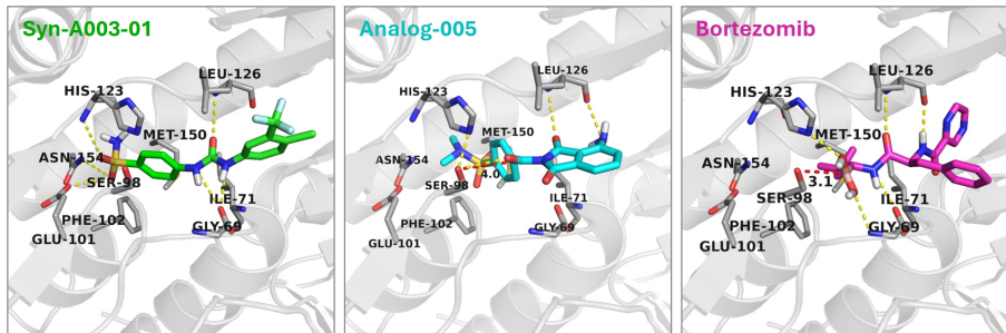
Fig. 5 Proposed binding modes of Syn-A003-01, Analog-005, and Bortezomib against ClpP. ClpP complex 5DZK is presented in grey cartoon. Syn-A003-01, Analog-005, and the reference compound Bortezomib are shown in green, cyan, and magenta sticks, respectively. The yellow dashed lines indicate hydrogen bonds. The red dashed lines with numbers denote distances between atoms.
