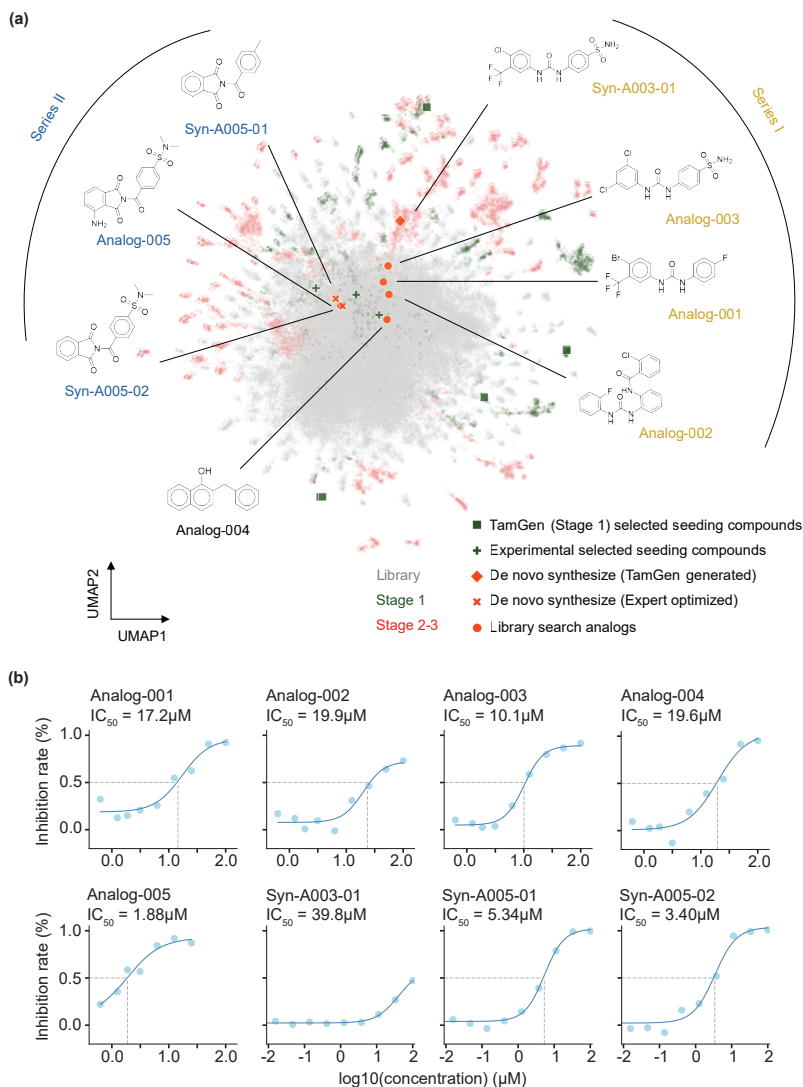
Fig. 4 Visualization and experimental validation on designed compounds. (a) UMAP visualization of library compounds and key compounds identified from the Design-Refine-Test pipeline with TamGen. Gray (background): 100K compounds sampled from library. Green (background): 2,612 compounds generated at Stage 1. Red (background): 8,365 compounds generated at Stage 2. Square and plus markers in green: seeding compounds used for Stage 2 generation. Circle, cross, and diamond markers in orange red: compounds subjected to IC_{50} determinations, stratified into 3 clusters based on molecular scaffold groups. (b) Dose-response assays for eight compounds with DMSO as a control. See methods for details of curve fitting and IC_{50} determination.
