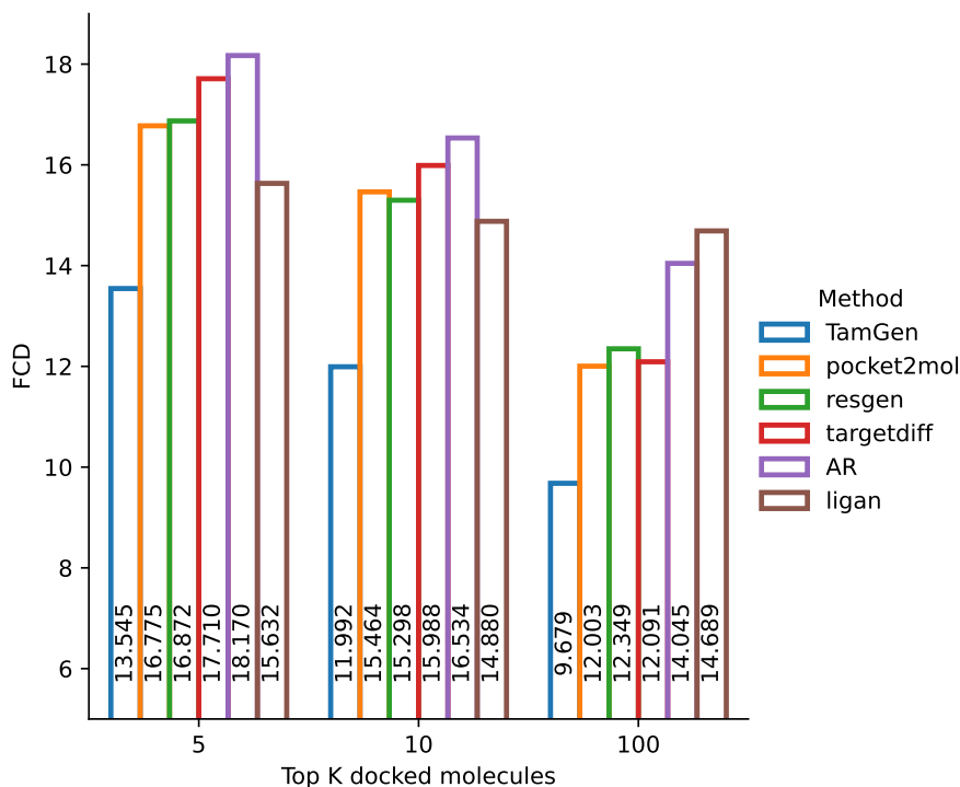
Fig. S4 The Fréchet ChemNet Distance (FCD) similarity [65] scores between FDA-approved drugs and compounds produced by different methods. FCD is a metric that quantifies the distributional dissimilarities between two compound sets, referred to as group A and group B. In this context, group A comprises all FDA-approved drugs, while group B includes compounds generated through various methods. A lower FCD score indicates a closer distribution of the generated compounds to the FDA approved drugs, signifying their similarity. TamGen demonstrates the capability to generate compounds that are most akin to FDA-approved drugs, as evidenced by the lowest FCD scores.
