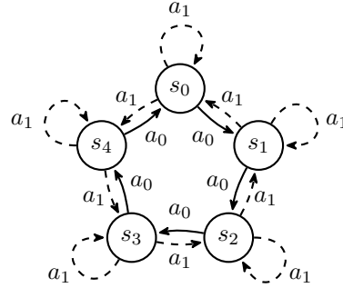
Figure 9: The five-state circular CMP. Agents start from state s_0 and take action a_i ( i = 0, 1 ). At every state s_i , choosing a_0 convergence transits to the next state s_{(i+1) \bmod 5} , forming circular transitions. At every state s_i , choosing action a_1 transits to state s_{(i-1) \bmod 5} with a probability of 0.7 and stays in the same state with a probability of 0.3, forming the stochastic transitions. Appendix E.3 uses this simple CMP to study the convergence of the FB and the one-step FB algorithms.
