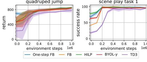
Figure 5: Fine-tuning pre-trained agents on downstream tasks. After offline pre-training, we conduct online fine-tuning on various methods using the same off-the-shelf RL algorithm (TD3). One-step FB continues to provide higher sample efficiency (+40% on average) during fine-tuning, as compared with the original FB method.
