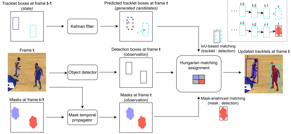
Figure 2. The overview of our proposed tracking pipeline. Top: Existing tracklet bounding box positions are considered as the tracker state from the previous frame, t-1 . Using Kalman filter, candidate tracklet positions are generated and considered as a predicted next state. Middle: Current frame t is passed to object detector. Then, initial association cost matrix is computed based on IoU between the bounding boxes of tracklet candidate positions and detections. Bottom: Mask temporal propagator takes the current frame t as an input and produces the masks, which are then considered as additional observation. The cost matrix is enriched with the information based on the matching between masks and detections. Finally, the cost matrix is passed to the Hungarian matching algorithm minimizing the association cost and the tracklets at frame t are updated with the matched detections.
