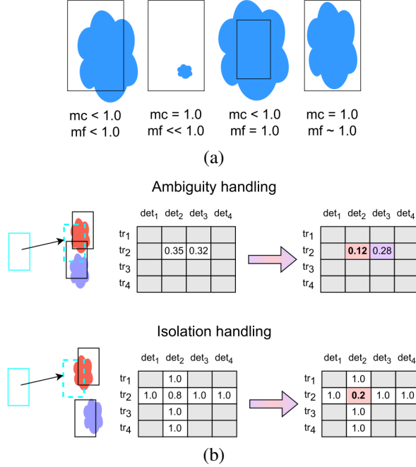
Figure 3. (a) Cases showing the differences in mc and mf values of a temporally propagated mask (in blue) within a bounding box. The most optimal case for the mask to provide a good guidance is the last one, where both mc and mf are as close to 1 as possible. (b) Ambiguity and isolation handling with the mask as a cue. Ambiguity occurs when the IoU-based costs are low and similar for more than one entry in a row (or column) of the cost matrix. Isolation occurs when relevant cost matrix entries contain too high values, not allowing for the association, and at the same time there is no ambiguity.
