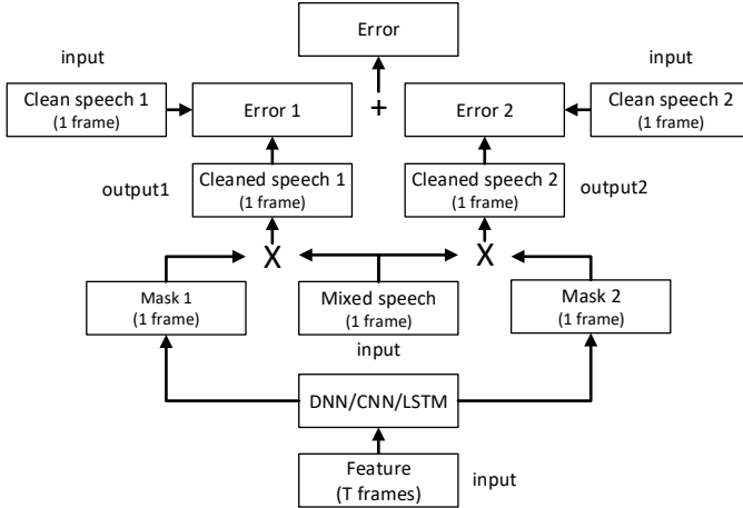
Fig. 1. The conventional two-talker speech separation model.
