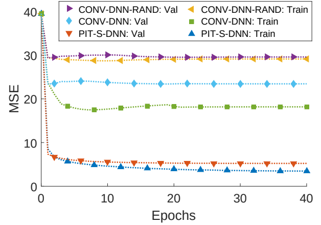
Fig. 3. MSE over epochs on the WSJ0-2mix training and validation sets with conventional training and PIT.
