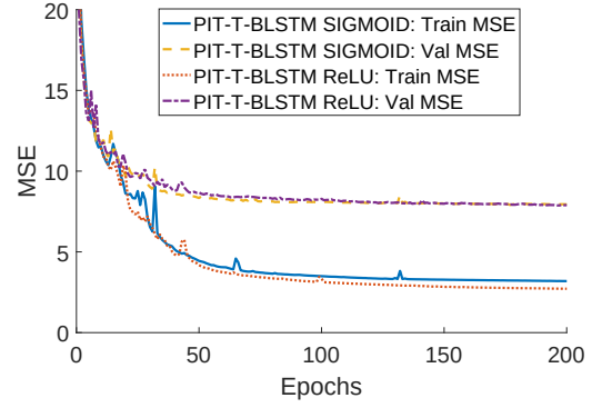
Fig. 4. MSE over epochs on the WSJ0-2mix PSM training and validation sets wit PIT-T.
