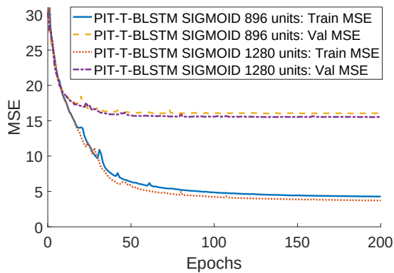
Fig. 5. MSE over epochs on the WSJ0-3mix NPSM training and validation sets wit PIT-T.
