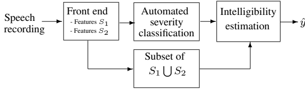
Figure 2: Block diagram of the proposed combined severity classification and intelligibility estimation system.
