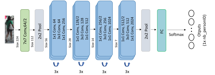
Fig. 2. ResNet-18 Architecture
