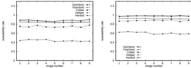
Figure 13: Repeatability rate for camera noise. \epsilon = 0.5 for the left graph and \epsilon = 1.5 for the right graph.
