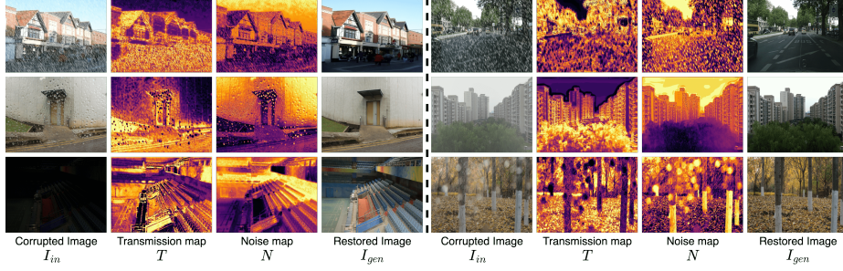
Fig. 5: Visualization of the learned Transmittance map T and Noise map N on different weather scenarios. T and N are re-normalized into [0, 1] for better visualization.
