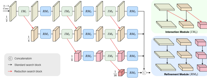
Fig. 3: Illustration of the multi-branch feature search, which contains three-stage of alternated Interaction Module IM and Refinement Module RM . In this work, we deploy the multi-branch learning after a standard 3 \times 3 convolution layer to decrease the resolution by half. Each black line represents a standard search block, and the red line denotes a reduction search block for downsampling. Taking the second stage IM_2 , RM_2 as an example, IM_2 generates an extra branch from the previous lowest-resolution branch by a reduction searching block (red line), while RM_2 further refine the features using cascaded standard search blocks (black line) within the same resolution.
