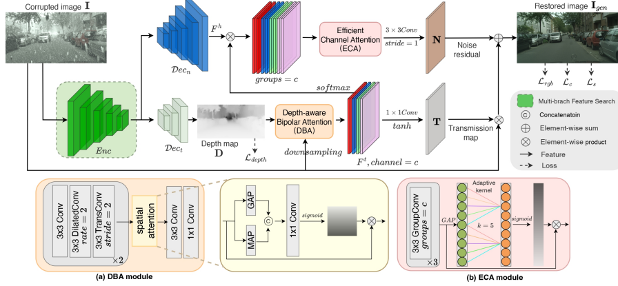
Fig. 2: The architecture of our Depth-aware Blind image decomposition Network (DeBNet). Given the corrupted image I_{noisy} with adverse weather, we extract the visual features via a searchable multi-branch encoder Enc (See Sec. 3.3 and Fig. 3). Then two decoder branches (Sec. 3.2) are deployed to progressively upsample the feature map with skip-connected features from the encoder. In particular, the transmittance decoder branch Dec_t is to predict the scene depth D . The noise branch Dec_n combines the learned attention weights with reconstructed high-resolution features. As shown in (a), we apply Depth-aware Bipolar Attention (DBA) module to compare the depth and the input image as the transmissivity map T . Besides, we also adopt an Efficient Channel Attention (ECA) module to fuse the depth and visual features to produce the depth-guided noise residual N as shown in (b). Finally, we fuse T , N , and I_{noisy} for joint restoration following Eq. (3).
