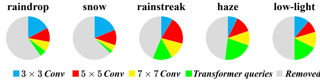
Fig. 7: Visualization of the searched architectures under different scenarios. For simplicity, we only show the averaged searching proportions in refinement modules when the feature size is scaled to 1/8 (see Fig. 3). More visualizations are given in the suppl.
