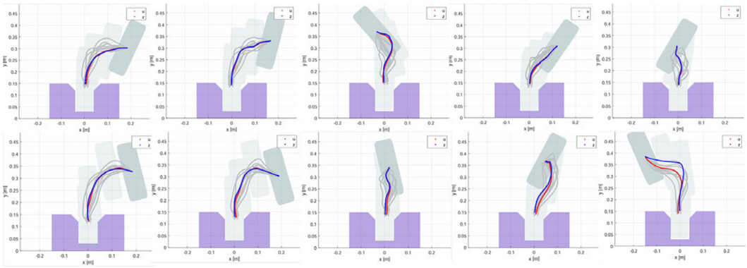
Figure 12. Variation of the initial position of the peg \mathbf{z}_0 .
