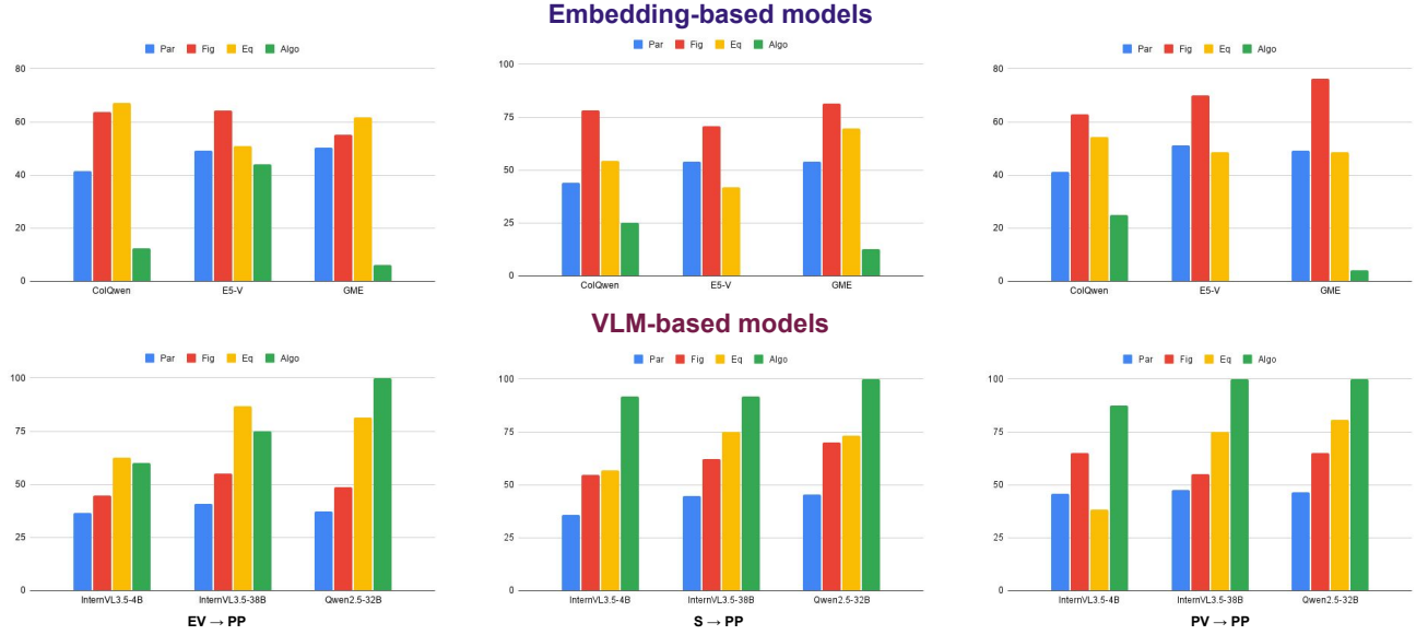
Figure 4. Illustrates the performance of embedding-based and VLM-based models across all three traversal settings ( EV \rightarrow PP , S \rightarrow PP , PV \rightarrow PP ). NDCG@2 scores are used for paragraphs, figures, and equations. For algorithms, recall is calculated using a threshold of 0.6.
