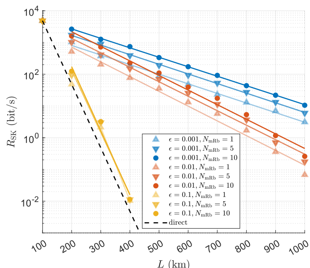
Fig. 4 | Average secret key rate ( R_{SK} ) as a function of distance ( L ) for different entanglement swap error probability ( \epsilon ), and number of auxiliary Rb memory atoms ( N_{mRb} ). Note that the total number of Rb memory atoms in each repeater station is 2N_{mRb} . The dashed black line presents the secret key rate with no repeaters but only a direct link between the two end nodes. The solid lines are linear fits excluding the data points for L = 100 km. The optimal number of repeater stations corresponding to each data point can be found in Supplementary Note 4. The simulation code is available in ref. 103.
