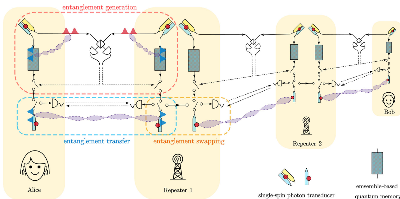
Fig. 1 | Structure of the quantum repeater chain architecture. The whole system contains two end nodes, Alice and Bob, connected by a series of repeater nodes. This figure depicts an example with two repeater nodes showcasing the key components involved. The yellow blocks represent the repeater nodes with the local devices depicted within. The protocol involves three main steps: entanglement generation, entanglement transfer, and entanglement swapping, as circled with dashed lines in different colors in the figure. The whole protocol harnesses two kinds of devices as
