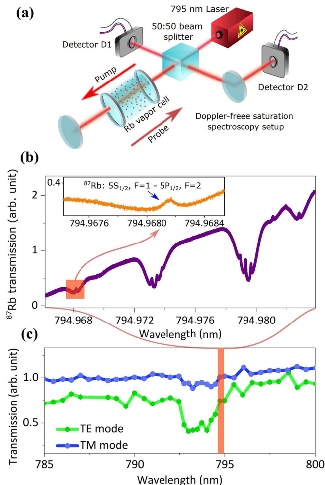
Fig. 3 | Compatibility of Rb and Tm- memory absorptions lines. a A simplified schematic of the Doppler-free saturation spectroscopy setup used to measure the absorption spectrum of rubidium. We use a laser with a continuously sweeping frequency, along with two light detectors (D1 to normalize the pump light, D2 to detect the probe light), to measure the absorption spectrum of the ^{87}\text{Rb} vapor. b Absorption spectrum of ^{87}\text{Rb} vapor. The inset shows an absorption peak corresponding to the [5^2S_{1/2}, F=1] \leftrightarrow [5^2P_{1/2}, F=2] transition, which is used in our single-spin photon transducer. c The absorption spectrum of Tm:LiNbO 3 . The orange bar indicates the wavelength range in (b), identifying the spectral overlap between the Tm-memory absorption and Rb photon transducer emission.
