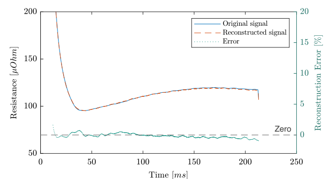
Fig. 8 Measured and reconstructed signal with means of an autoencoder network, with topology 450k - 15 - 450k
