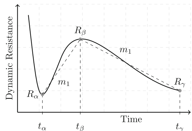
Fig. 4 Theoretical dynamic resistance curve, with selected features for the geometrical attributes approach, adopted from [9]
