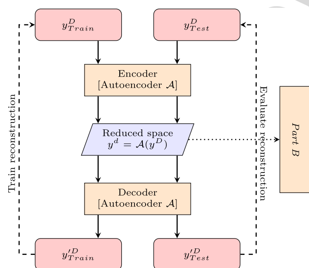
Fig. 7 Workflow c. Autoencoder training principle
