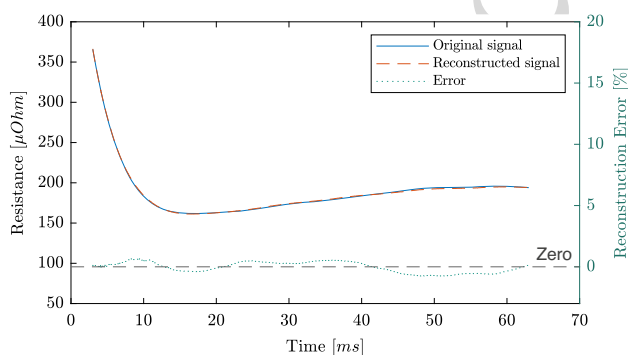
Fig. 11 Measured and reconstructed signal with means of an autoencoder network, with topology 450k - 15 - 450k for the current variation case
