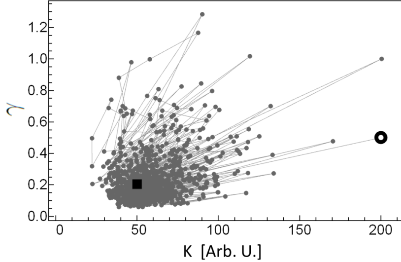
Figure 6: System dynamics in the phase space K - \gamma . The empty circle represents the initial state, while the square corresponds to the true parameter values used to generate the data.
