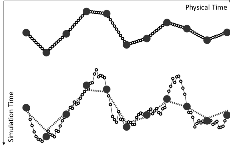
Figure 1: Simulated dynamics of a polymer chain with n + 1 = 11 data points (large filled circles) and j - 1 = 9 intermediate beads (small empty circles). All other parameters are discussed in Section 4. Top: initial state. The intermediate beads represent a linear interpolation to the data points. Bottom: polymer configuration after 1000 iterations of the propagation algorithm. The dotted line represents the initial configuration. It is evident that the new configuration is mostly determined by the dynamics of the low-mass intermediate beads, while the heavy-mass data points barely move from their initial positions.
