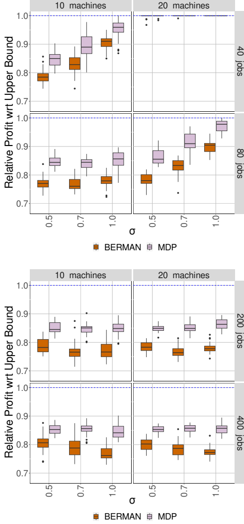
Fig. 5: Comparison of \mathcal{BERMAN} and \mathcal{MDP} .
