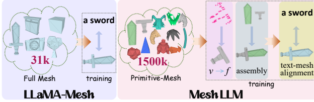
Figure 2. Differences between LLaMA-Mesh and MeshLLM. LLaMA-Mesh applies a single text-mesh alignment optimization strategy on only 31k available meshes. In contrast, our proposed MeshLLM leverages local mesh patches and thus expands the trainable data to 1500k, enhancing model performance through vertex-to-face prediction and local mesh assembly strategies.
