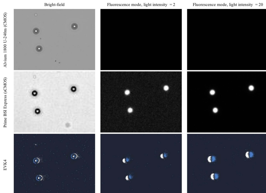
Figure 4. Microscopic imaging captured by Alvinum 1800 U-240 m (CMOS), Prime BSI Express (sCMOS) and EVK4 under varying illumination conditions. The first column on the left illustrated the images captured under a bright-field. The second column indicated the images taken in a fluorescence mode with light intensity set on 2 in the blue light region. The third column illustrated the images taken with light intensity set on 20 in the blue light region.
