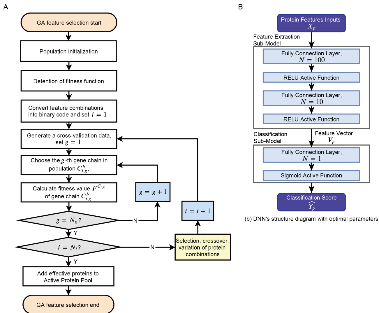
Figure S5. Structures of artificial neural network models.
