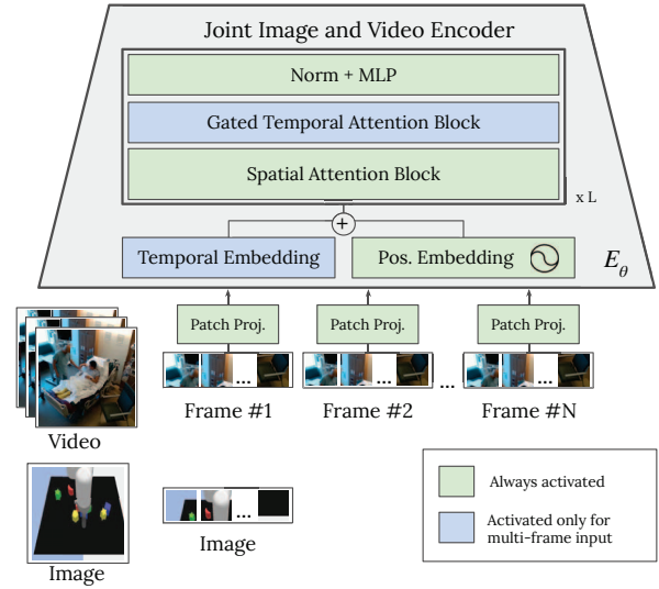
Figure 2. Our Visual Encoder, E_\theta . We use a lightweight gated temporal attention mechanism that activates only for multi-frame inputs, allowing us to use most of the model parameters for both image and video inputs while still enabling cross-frame temporal attention within the visual encoder when desired. We use sinusoidal positional embeddings for effective MAE reconstruction.
