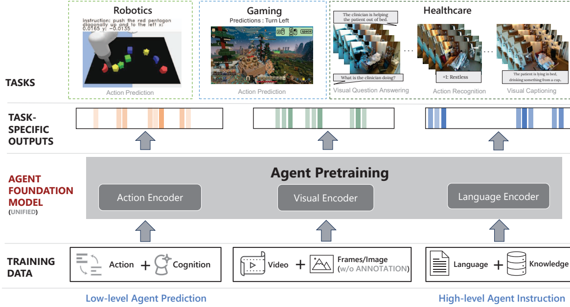
Figure 1. Overview of our Interactive Agent framework. Our foundation model is designed to process multi-modal information that conveys various levels of abstraction. This approach facilitates a comprehensive understanding of the context and environment, thus ensuring that actions are coherent. By training on a variety of task domains and applications, we develop a versatile foundation model that can be fine-tuned for executing optimal actions in a variety of contexts.
