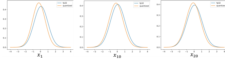
Fig. 2: The distribution shift caused by the accumulated quantization error. We gather the statistics of sub feature maps at timestep 1, 10, and 20.
