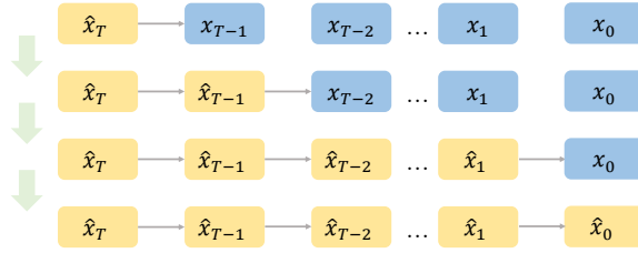
Fig. 1: Progressive calibration for activations. The yellow bar means the activation has been quantized. We quantize the activations at step t with all the previous steps quantized, which considers the accumulated quantization error across timesteps.
