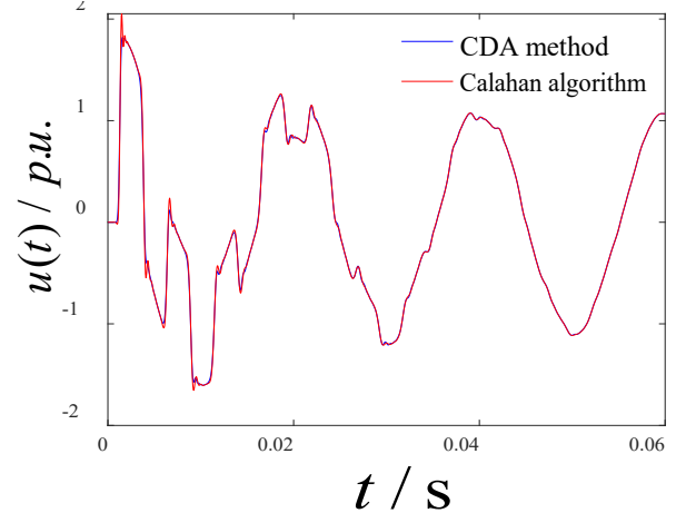
(c) Terminal voltage waveforms calculated by CDA method and Calahan algorithm
