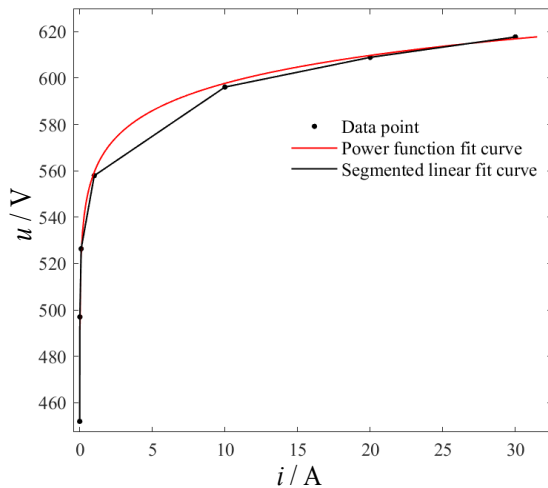
FIGURE 1. S10K250 Varistor volt-ampere characteristic curve.
