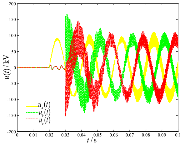
(b) Three-phase high-voltage side voltage waveforms
