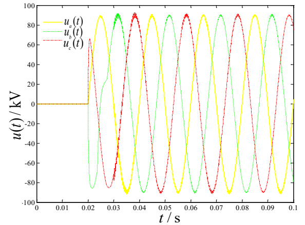
(b) Three-phase high-voltage side voltage waveforms
