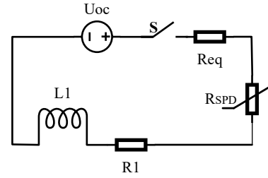
FIGURE 4. Thevenin equivalent circuit diagram during cooler shutdown.
