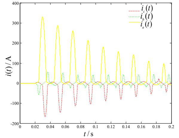
(a) Three-phase excitation inrush waveforms
