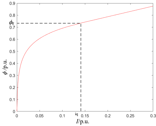
FIGURE 9. Function fitting model of excitation curve.
