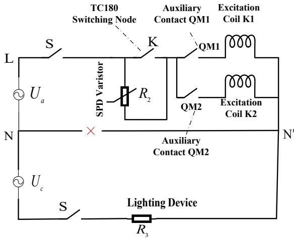
FIGURE 2. Starting and stopping control circuit of converter transformer cooler.
