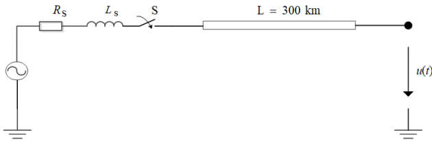
FIGURE 12. Schematic diagram of a transmission line without load being switched-in suddenly.
