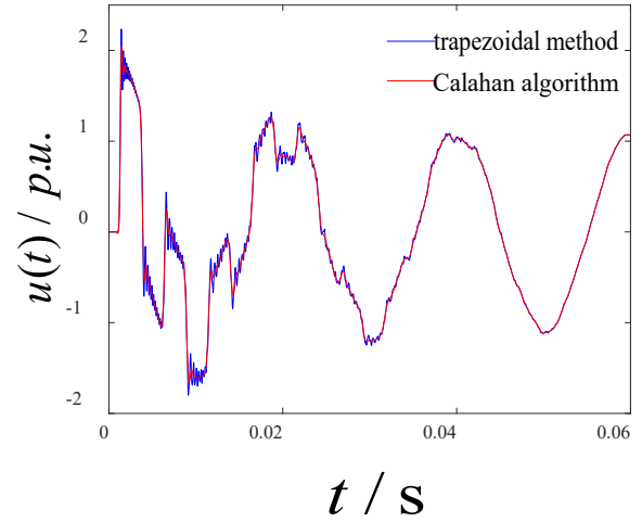
(a) Terminal voltage waveforms calculated by implicit trapezoidal method and Calahan algorithm
