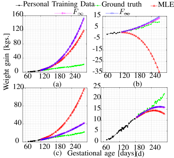
Fig. 2: Federated learning generates (a) worst (subject id #14) and (b) best result (subject id #47) with limited personal data up to 120 days when only 10 users have participated initially. Performance for the subject id #14 can be seen improving when (c) 70 users participated in federated learning or when (d) the availability of personal-data increased (up to 180 days).
