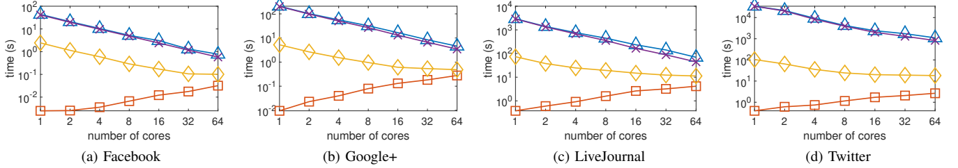
Fig. 6: Running time of DiIMM for IM under IC model using a multi-core server.
