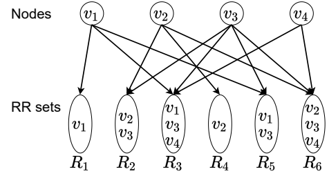
Fig. 2: RR sets and maximum coverage.
