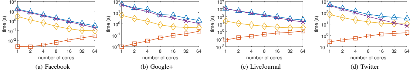
Fig. 9: Running time of DiIMM for IM under LT model using a multi-core server.
