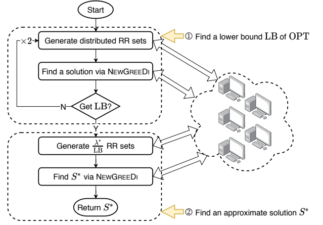
Fig. 4: Flowchart of DiIMM.
