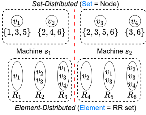
Fig. 3: Comparison between set-distributed approach and element-distributed approach.
