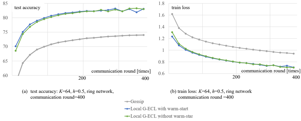
Fig. 7. Convergence curves using (a) test accuracy and (b) train loss using Local G-ECL with/without warm-start, and Gossip as a reference. Associated hyper-parameters are set as (h, K, R) = (0.5, 64, 400) .
