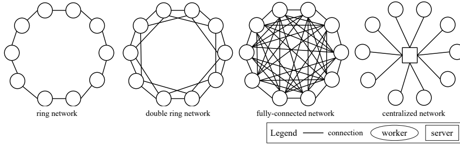
Fig. 5. Network topologies of ring ( |\mathcal{N}_i| = 2 ), double ring ( |\mathcal{N}_i| = 4 ), fully-connected ( |\mathcal{N}_i| = 9 ), and the centralized network.
