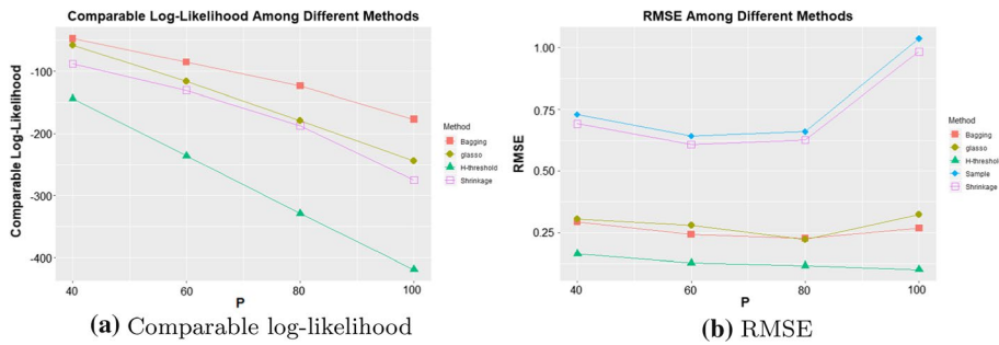
Fig. 4 a For comparable log-likelihood \ell_t , our Bagging estimator beats others significantly across all values of p . b For RMSE, the Bagging estimator is second only to the hard-threshold method, which has the worst performance from the perspective of \ell_t
