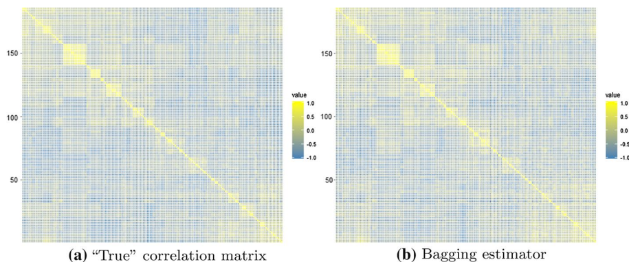
Fig. 5 a Heat map of the sample correlation matrix of the full 139 samples, which is viewed as “true” correlation matrix for comparison. b Heat map of the Bagging estimator on a subset of 70 samples
