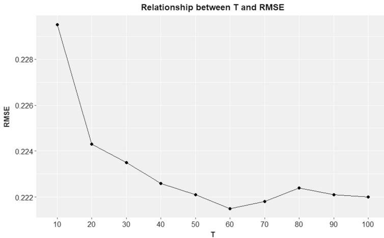
Fig. 2 The RMSE of Bagging estimator decays with the increase of T at the beginning and then seemingly converges to a stable level
