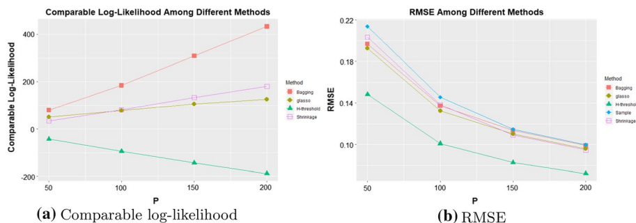
Fig. 3 a For comparable log-likelihood \ell_N , our Bagging estimator beats others significantly across all values of p . b For RMSE, the Bagging estimator is second only to the hard-threshold method, which has the worst performance from the perspective of \ell_N
