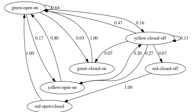
Fig. 9. Aggregated multi-sensor behavior with three abnormal states
