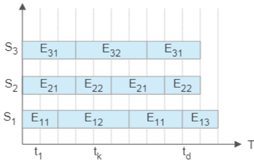
Fig. 1. Illustration of multi-sensor sensor streams
