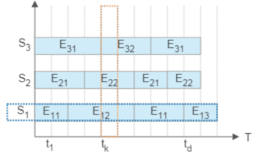
Fig. 2. Illustration of event behavior within sensor and across sensors
