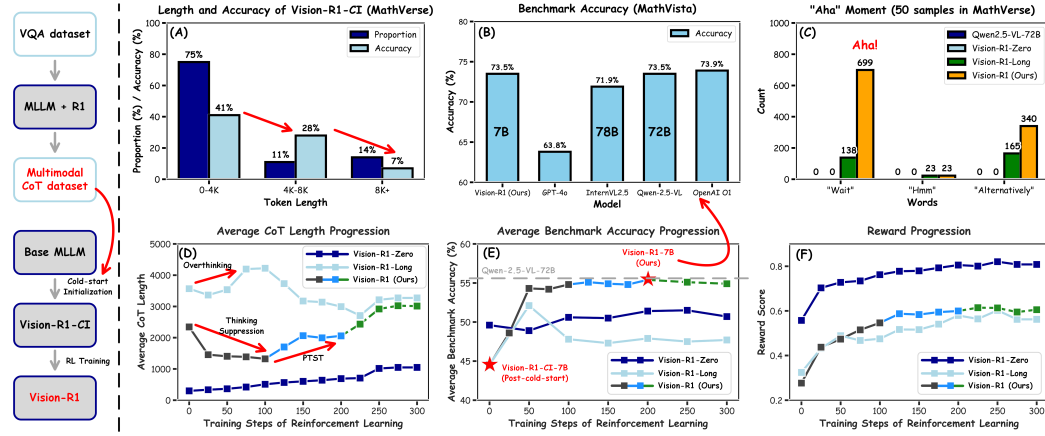
Figure 1: Left panel: Our Vision-R1 Pipeline. We first use the existing MLLM and DeepSeek-R1 to obtain a high-quantity Multimodal CoT dataset, which is used as the cold-start initialization data for the base MLLM to obtain the post-cold-start Vision-R1-CI, and then we perform the RL training on Vision-R1-CI to obtain the reasoning MLLM, Vision-R1. Right panel: We observe that directly applying RL to MLLMs fails to effectively incentivize strong reasoning capability (see (C) and (D)). Vision-R1-Zero, trained via RL without prior initialization, struggles to generalize from limited data (see (E), (F), notably, Vision-R1-Zero was applied in format reward function). Vision-R1-CI faces the Overthinking Optimization Problem, favoring shorter CoT reasoning, where correct reasoning processes mostly focus on the shorter CoT reasoning sequences (see (A)). During subsequent RL training, we observe a lengthening of reasoning steps but a decline in performance (see (D) and (E)), making optimization particularly challenging. For Vision-R1, it initially shortens CoT to refine the right thought process under RL training. PTST enables Vision-R1 to progressively acquire a more complex reasoning process (see (C), (D), and (E)) to improve the performance, such that our Vision-R1 with 7B parameters achieves comparable performance to the 70B+ strongest MLLMs (see (B)). Note that Vision-R1 used various colored lines to indicate the different stages in PTST.
