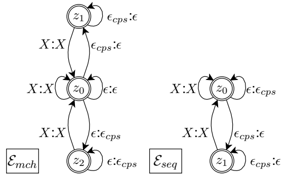
Figure 2: Matching and sequential \epsilon -filter
